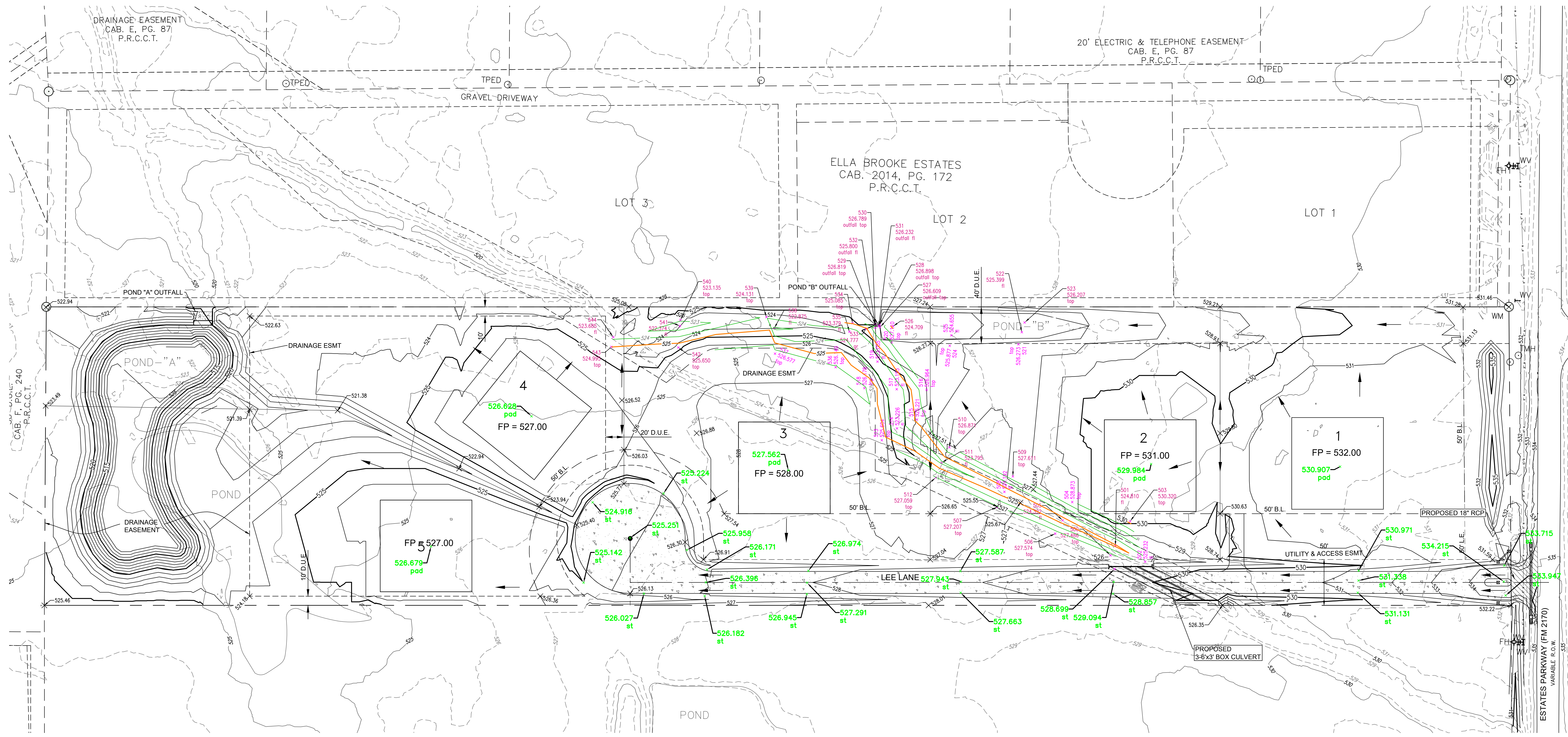
GRADING PLAN EXHIBIT THE FARMSTEAD COLLIN COUNTY, TEXAS
