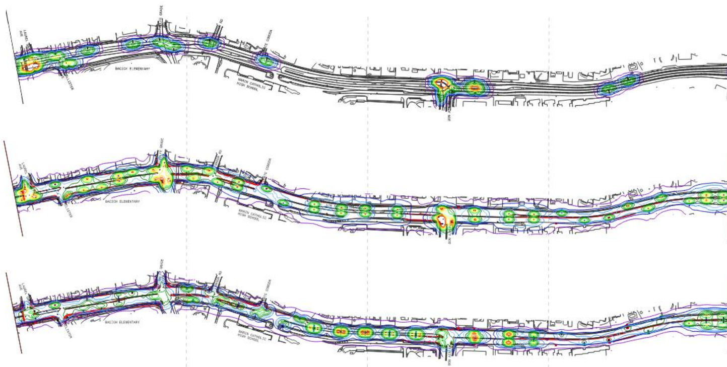
Sir Francis Drake Boulevard Photometrics - Sheet 2 of 3
