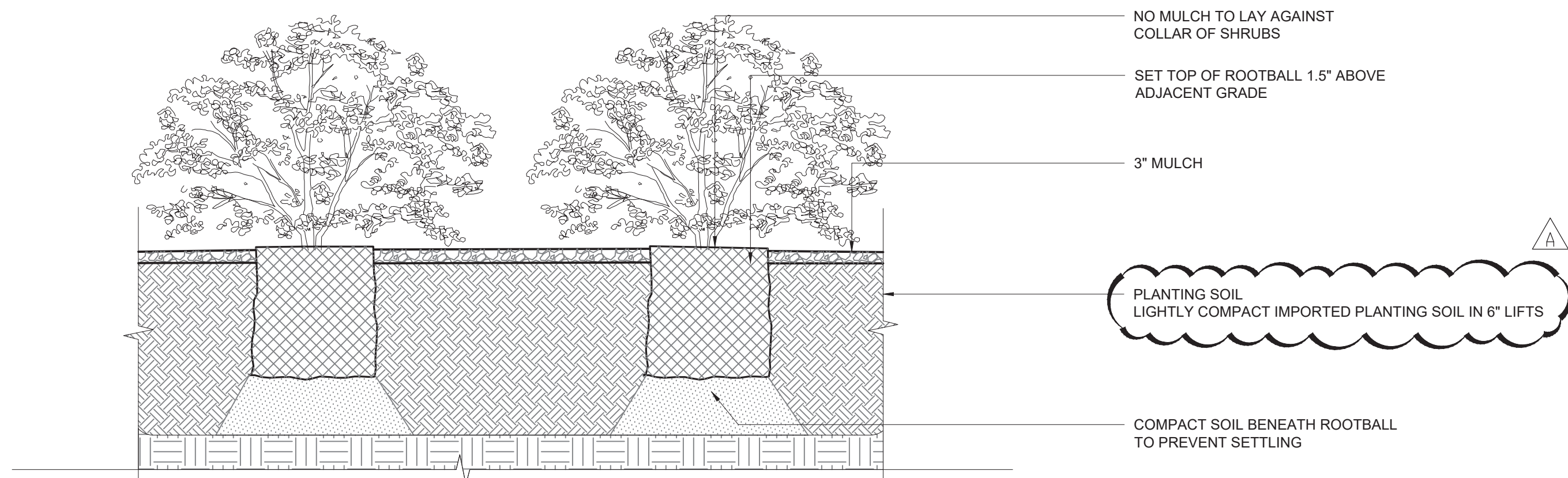
2 SHRUB PLANTING IN IMPORT SOIL AREAS
