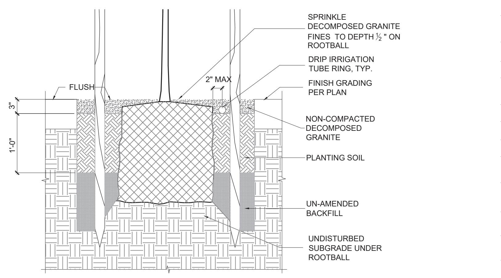
8 TREE PLANTING AT DG TREE WELL
