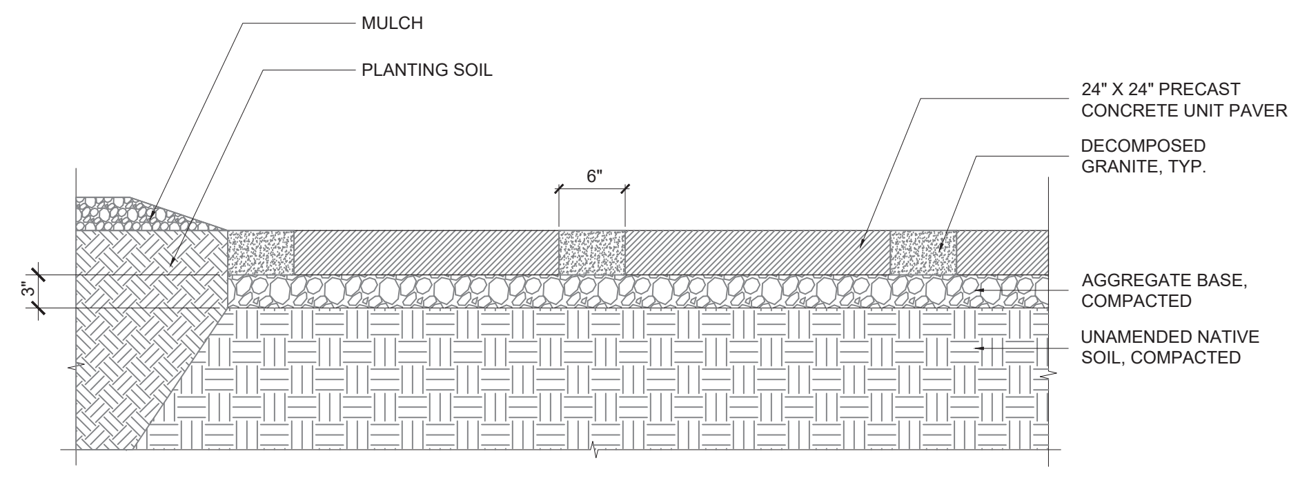
4 CONCRETE UNIT PAVER WITH DG INFILL
