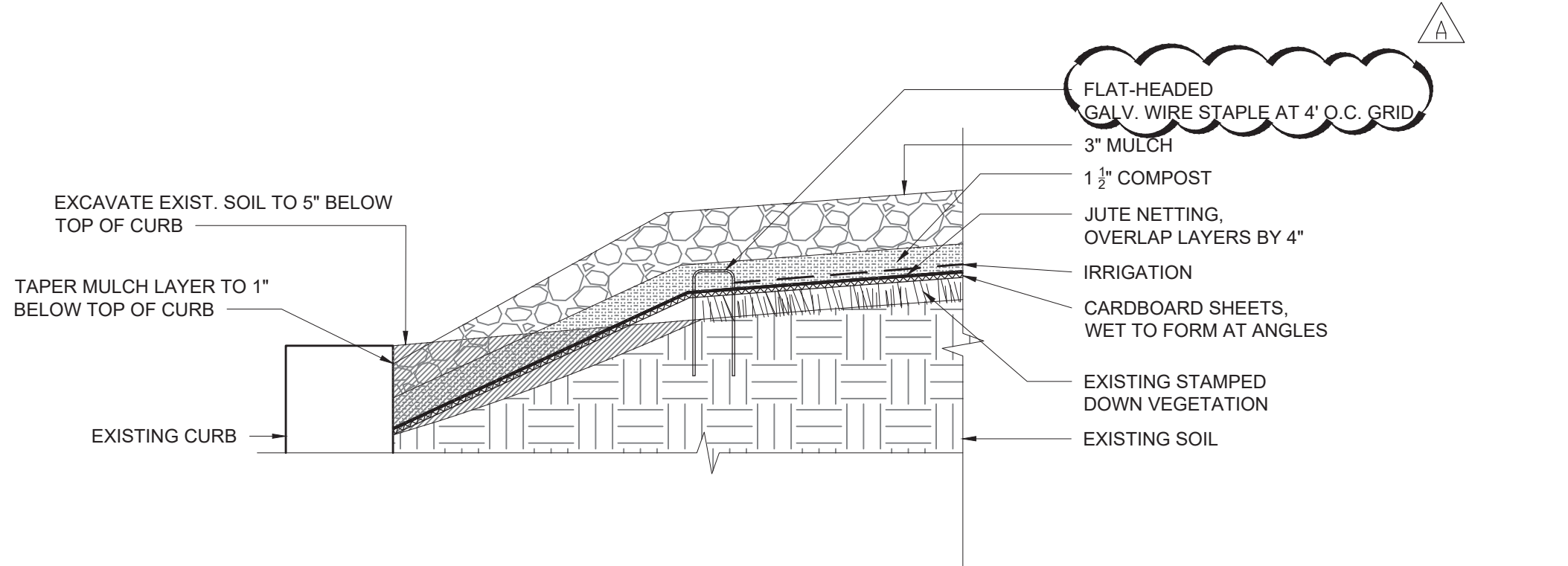
5 SHEET MULCH DETAIL
