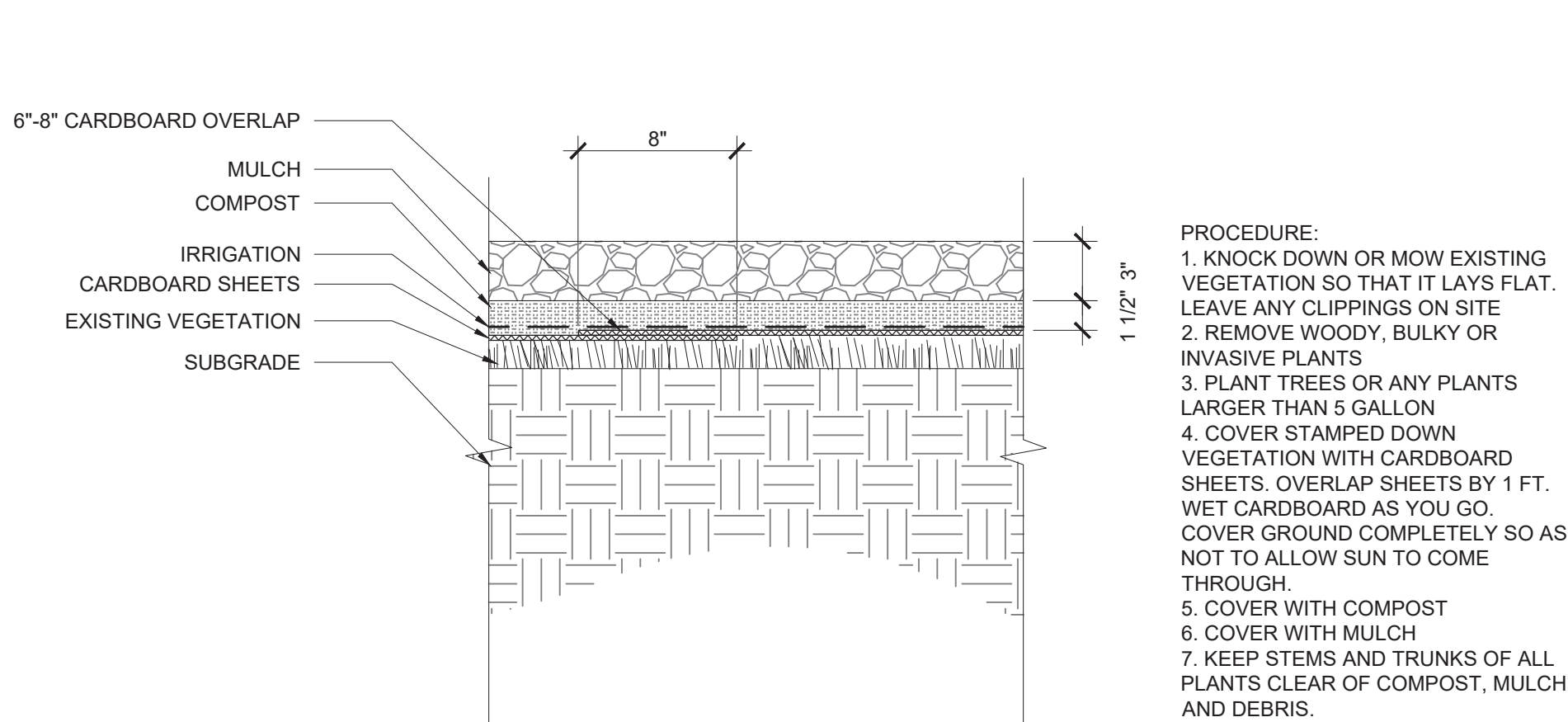
5 SHEET MULCH DETAIL
