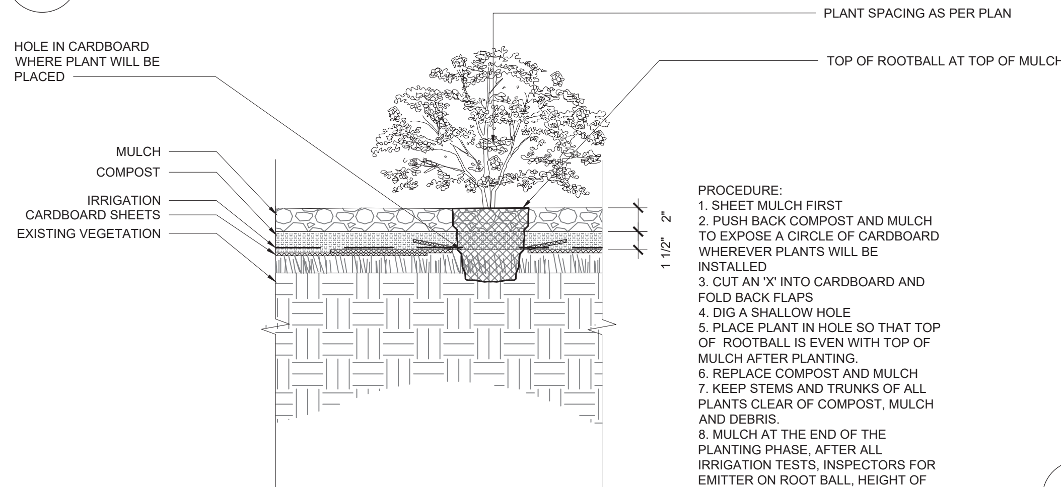
6 SHEET MULCH DETAIL AT MEDIANS WITH MOUNDED SOIL
