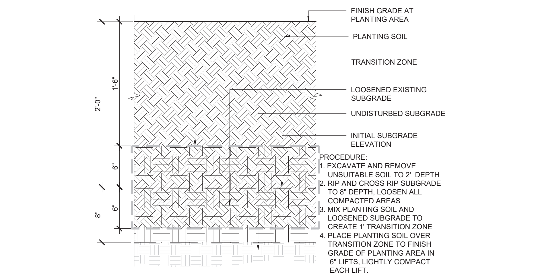
3 SOIL PREPARATION FOR IMPORT SOIL AREAS
