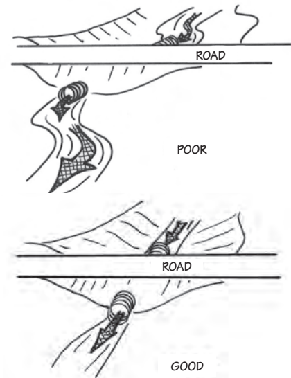
Culvert alignment under road
