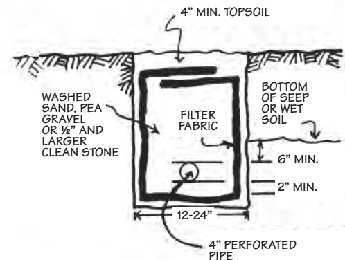
Subsurface drain
