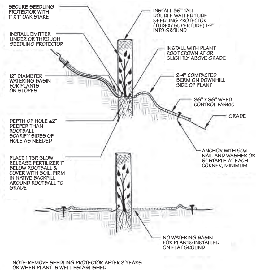
Planting details for slopes and flat ground
