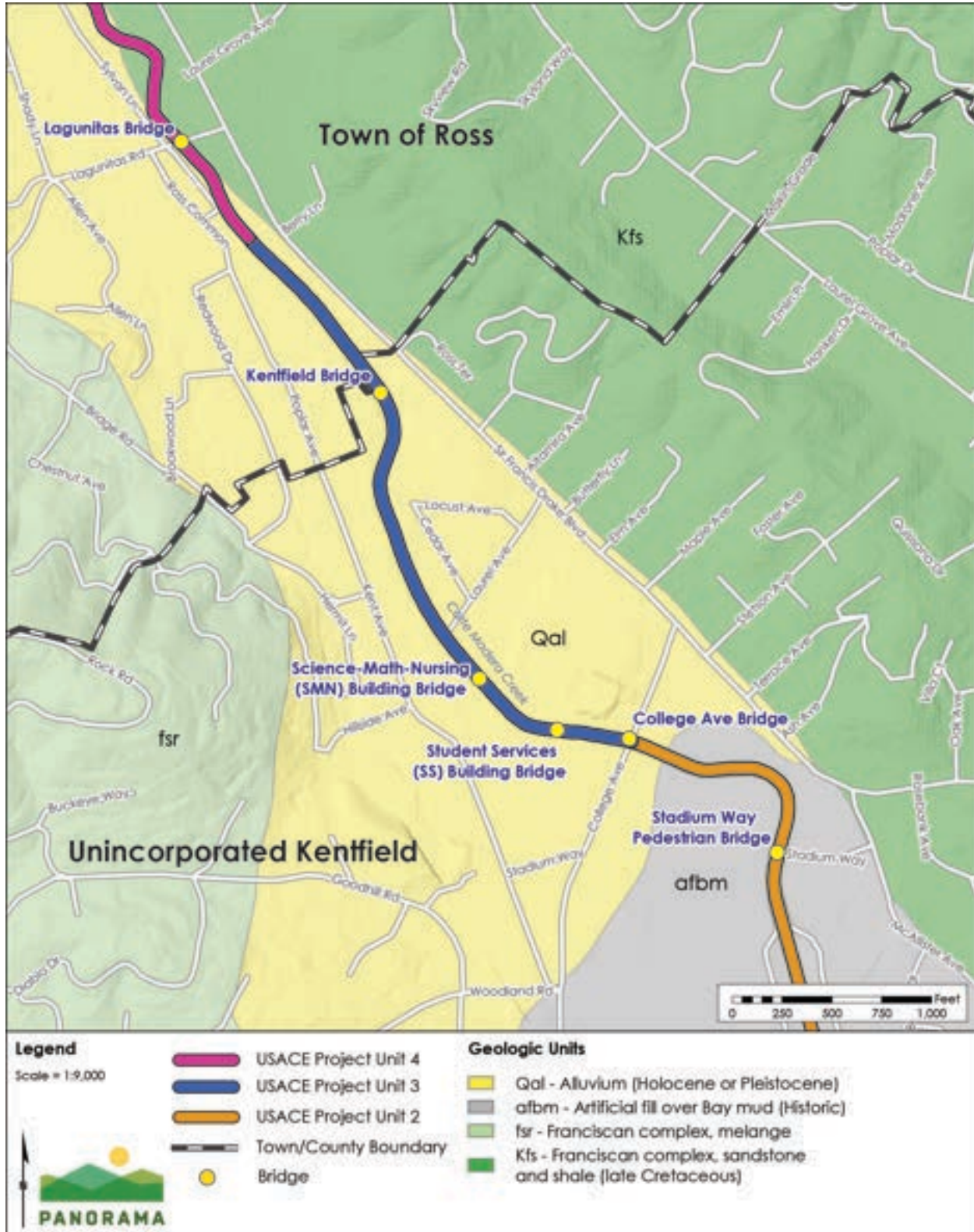
Figure 3.6-1 Geologic Units
