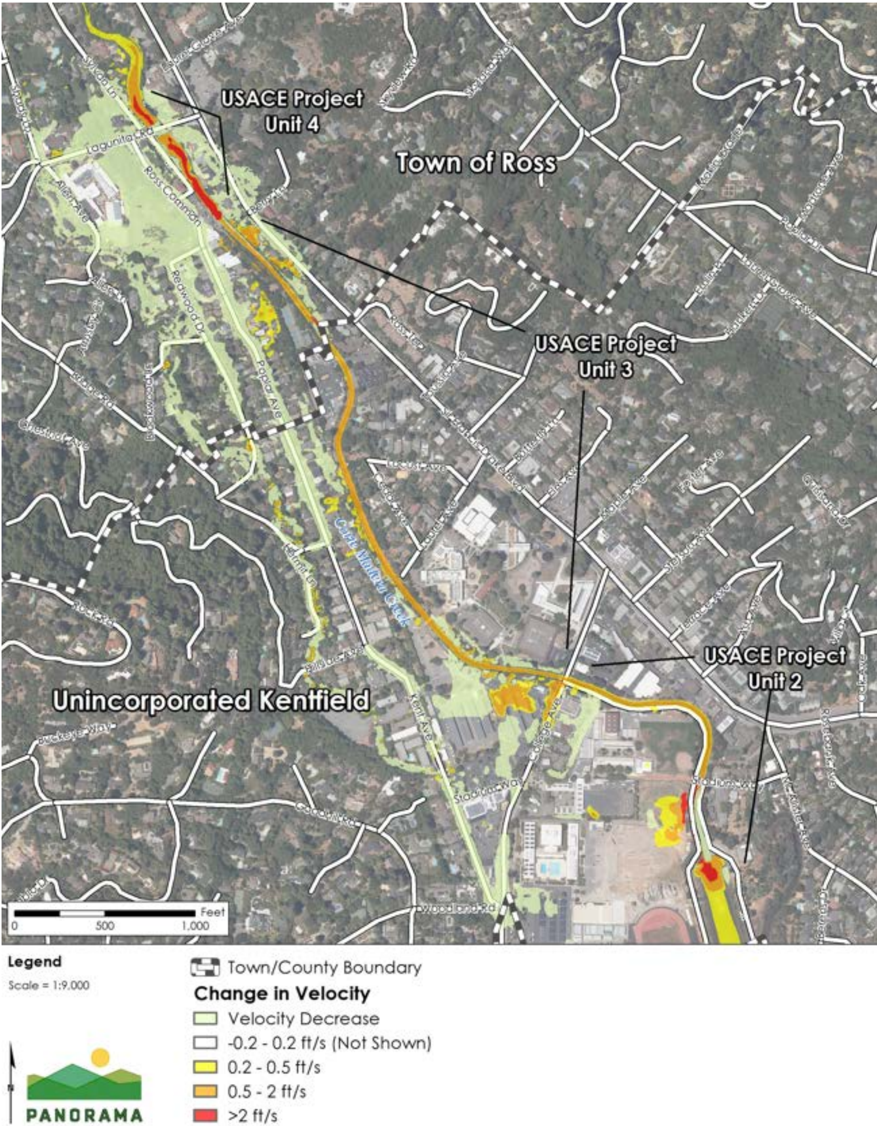
Figure 5.3-4 Alternative 1 Changes in Velocity from Future Conditions - 100-Year Flood Event
