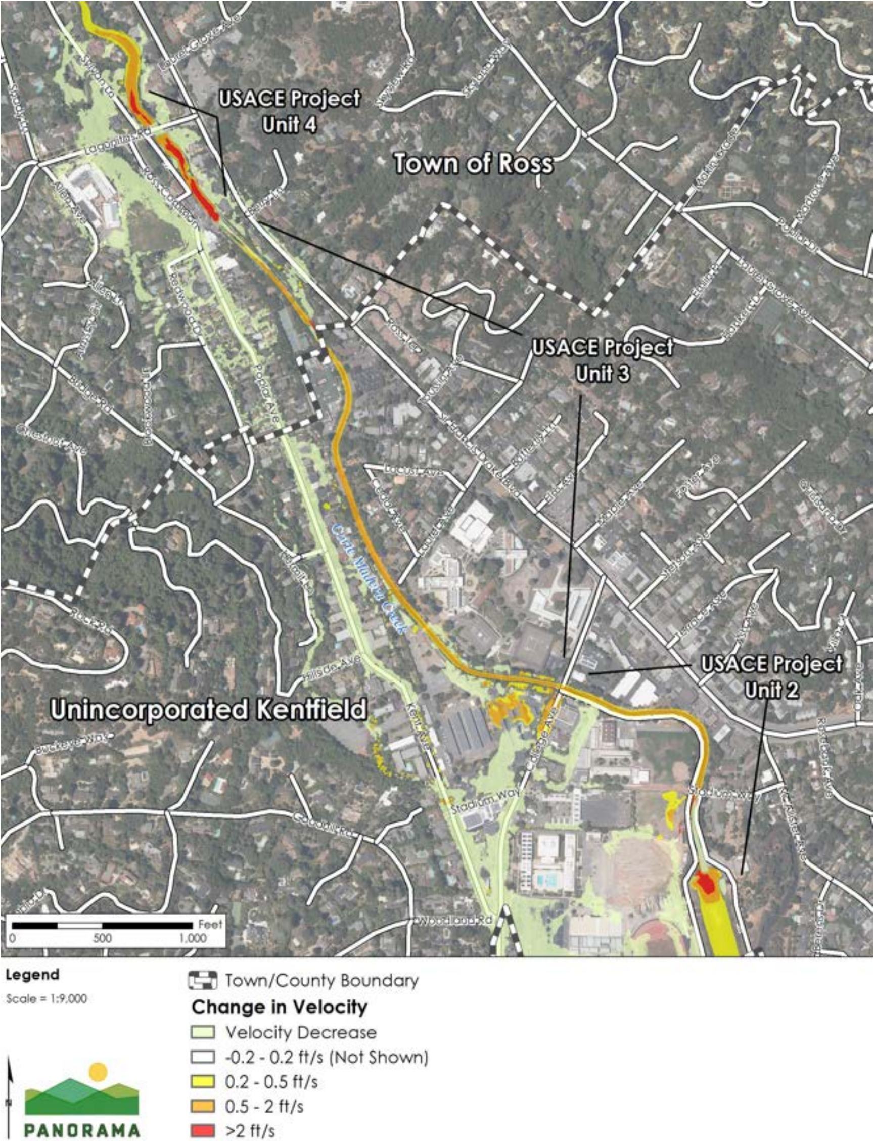
Figure 5.3-3 Alternative 1 Changes in Velocity from Future Conditions - 25-Year Flood Event
