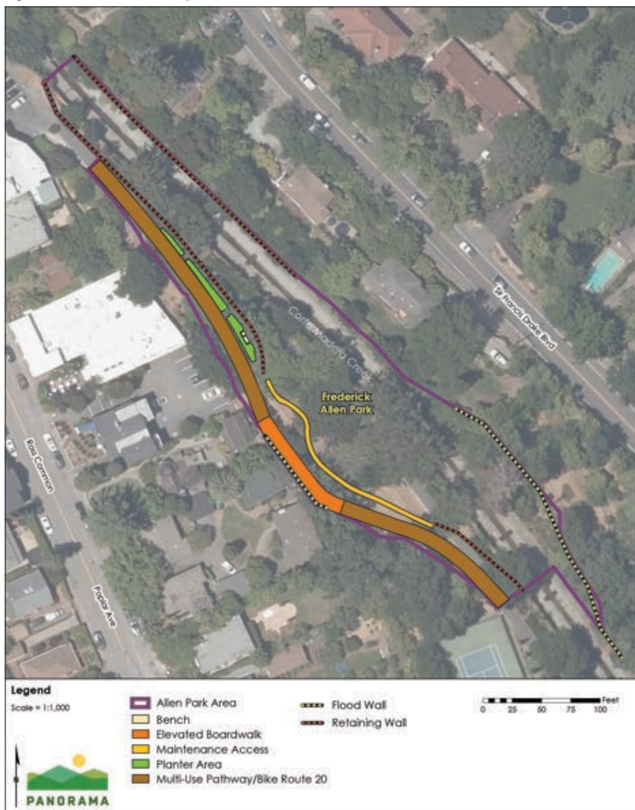
Figure 5.3-9 Alternative 2 Layout
