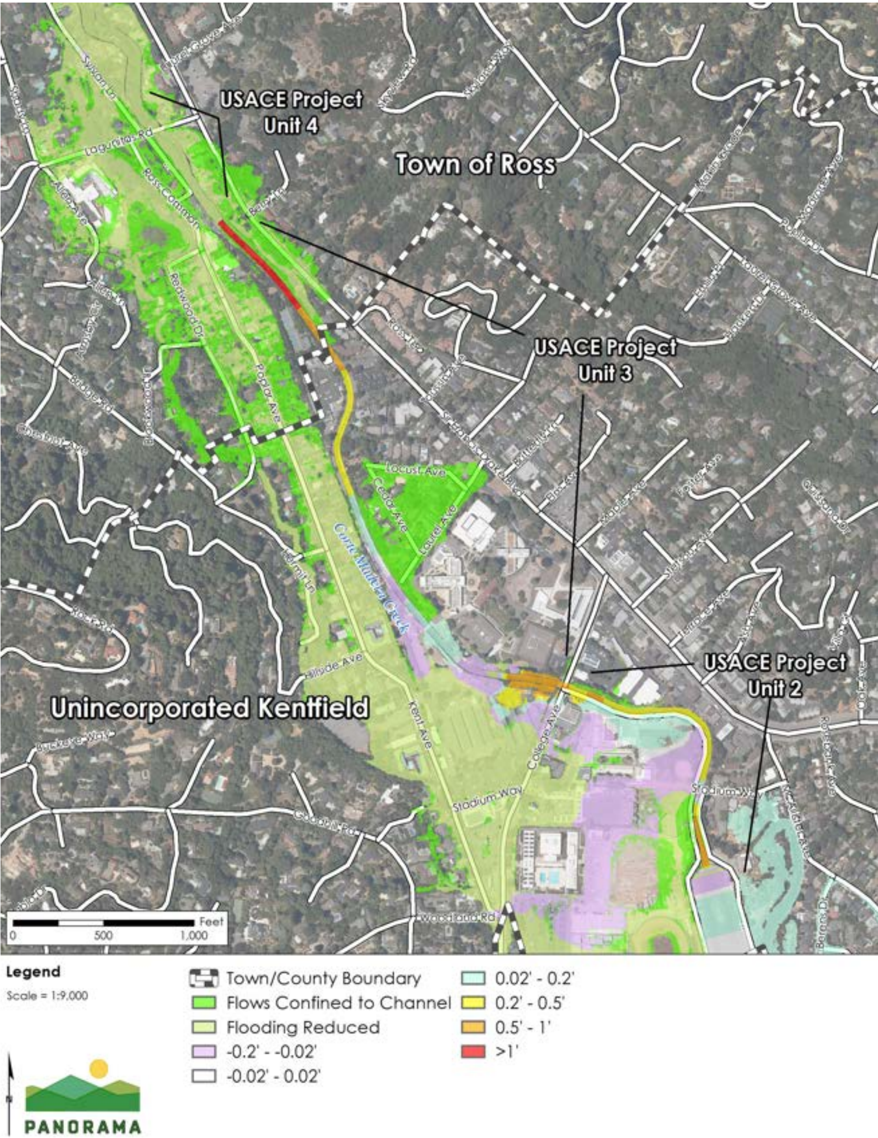
Figure 5.3-6 Alternative 1 Changes in Water Surface Elevation, Future Conditions, 25-Year Flood Event
