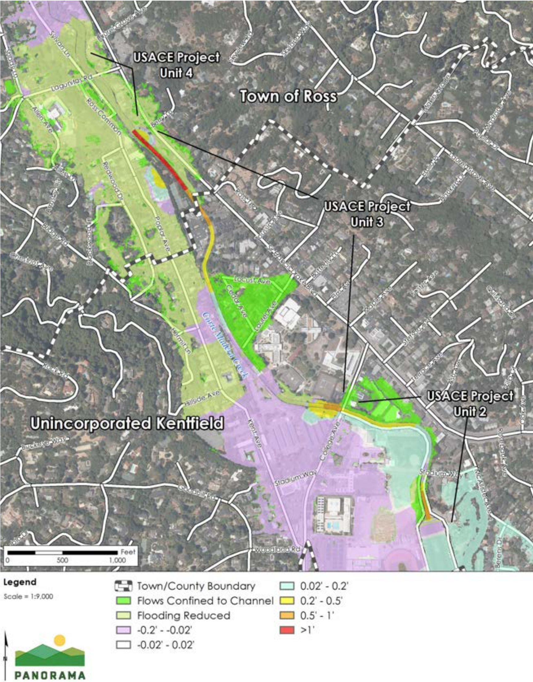
Figure 5.3-7 Alternative 1 Changes in Water Surface Elevation, Future Conditions, 100-Year Flood Event
