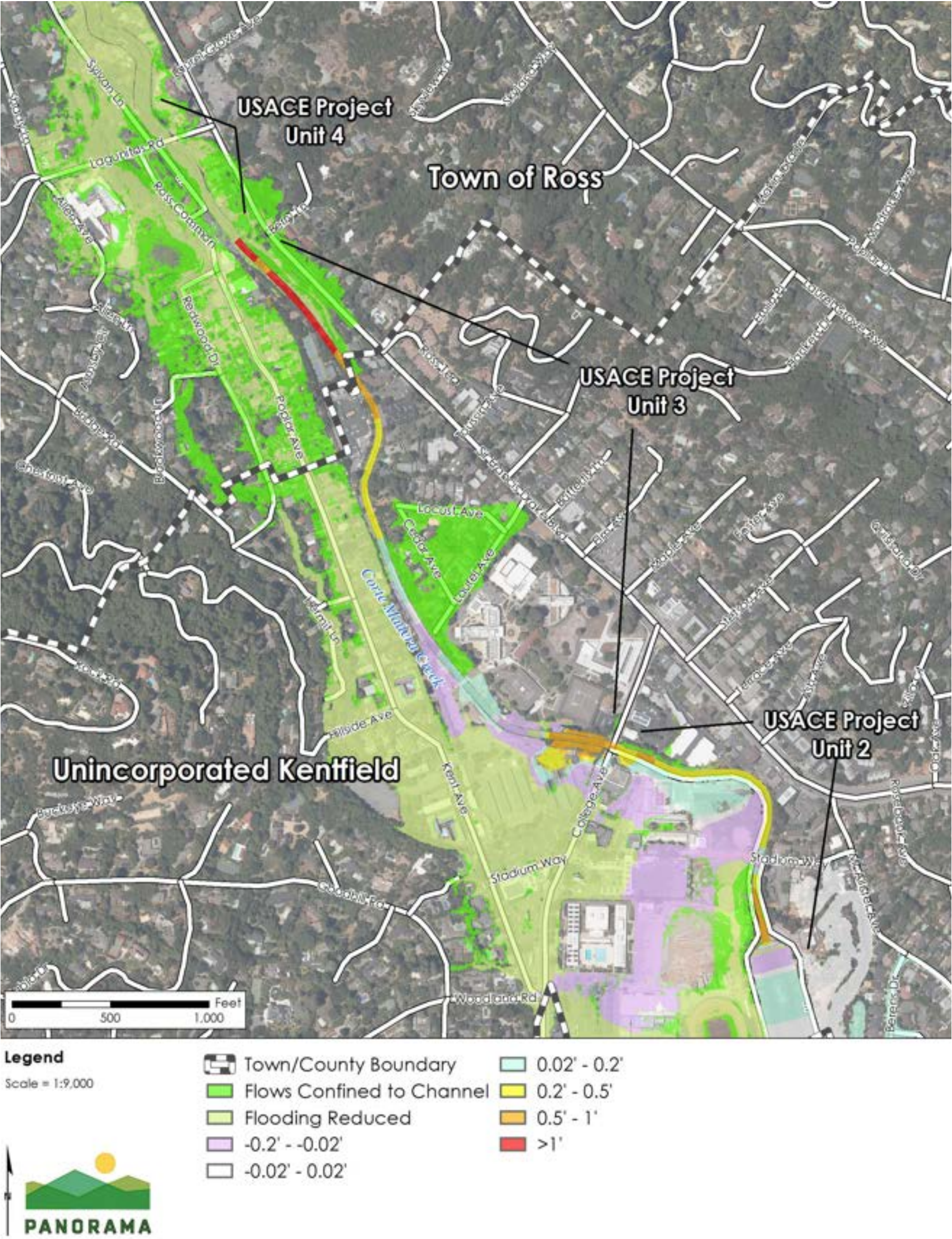
Figure 3.9-8 Project Changes in Water Surface Elevation from Future Conditions, 25-Year Flood Event
