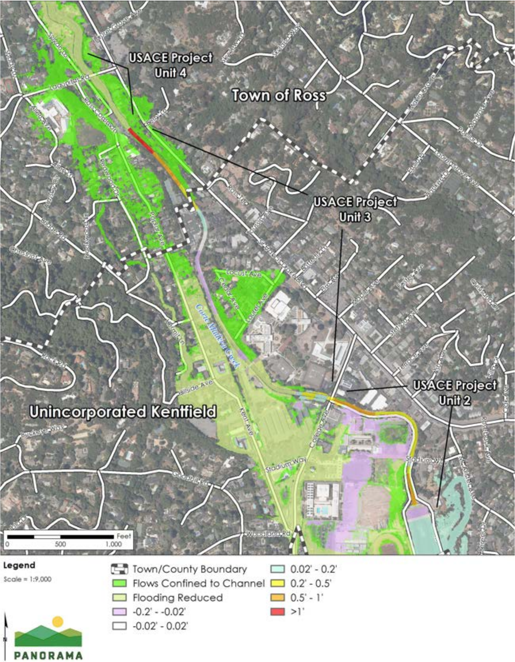
Figure 5.3-5 Alternative 1 Changes in Water Surface Elevation, Future Conditions, 10-Year Flood Event
