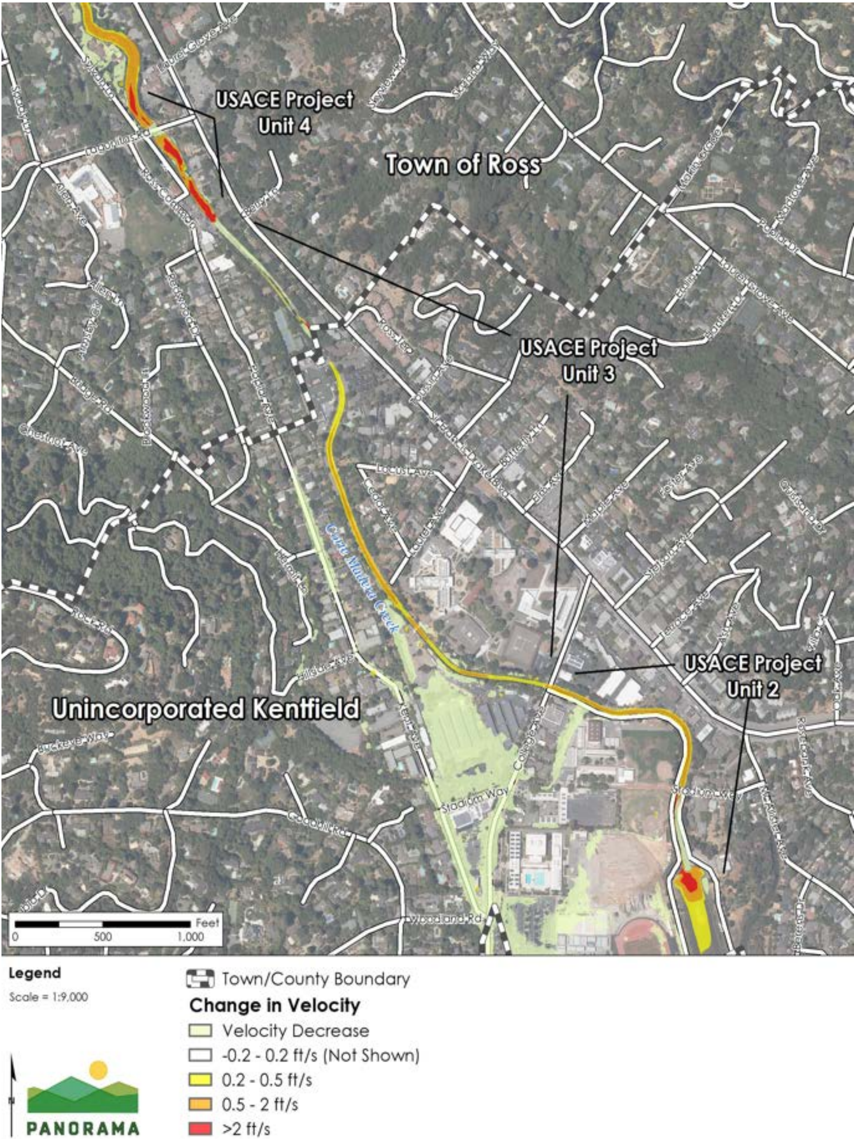
Figure 5.3-2 Alternative 1 Changes in Velocity from Future Conditions - 10-Year Flood Event
