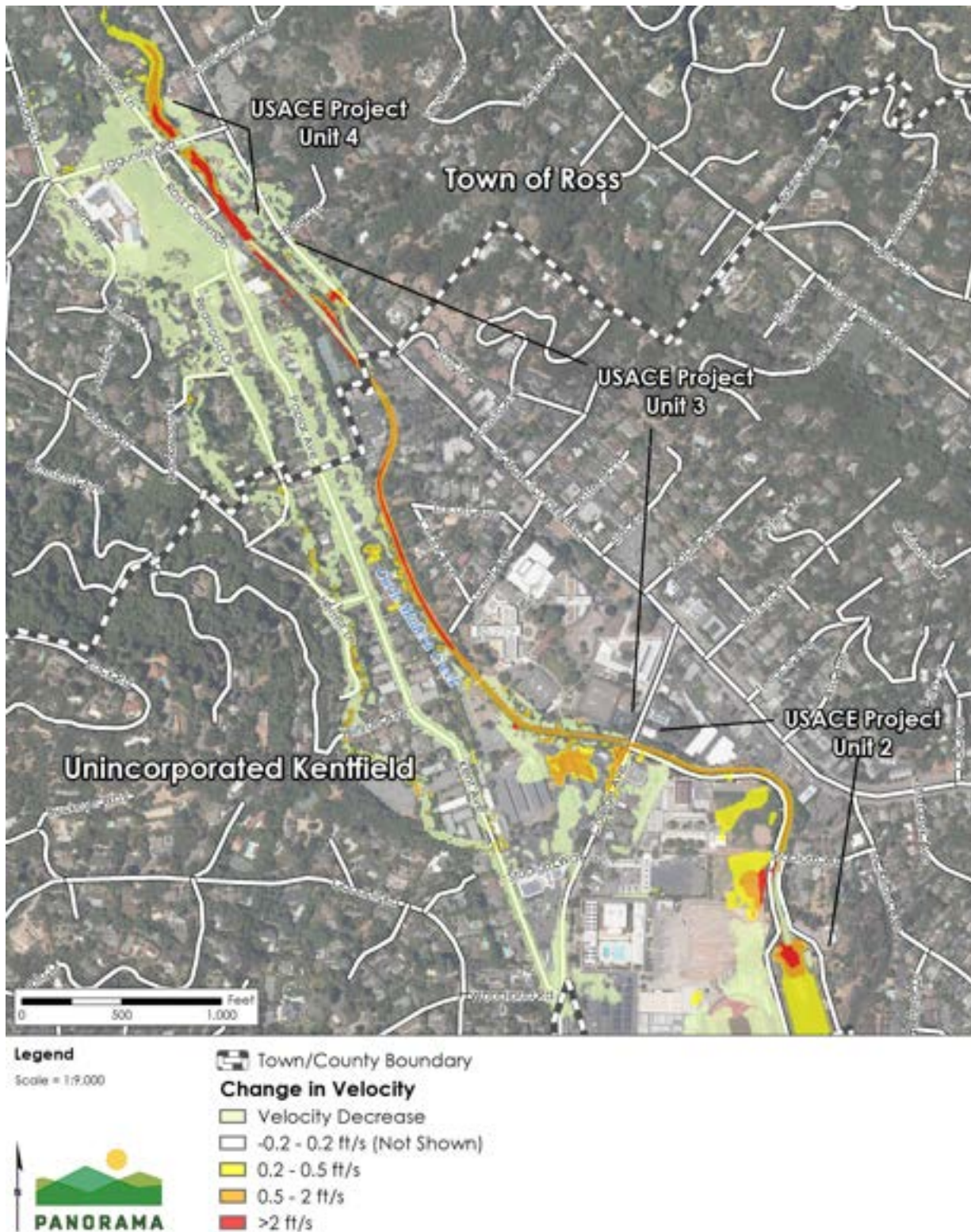
Figure 3.9-6 Project Changes in Velocity from Future Conditions, 100-Year Event
