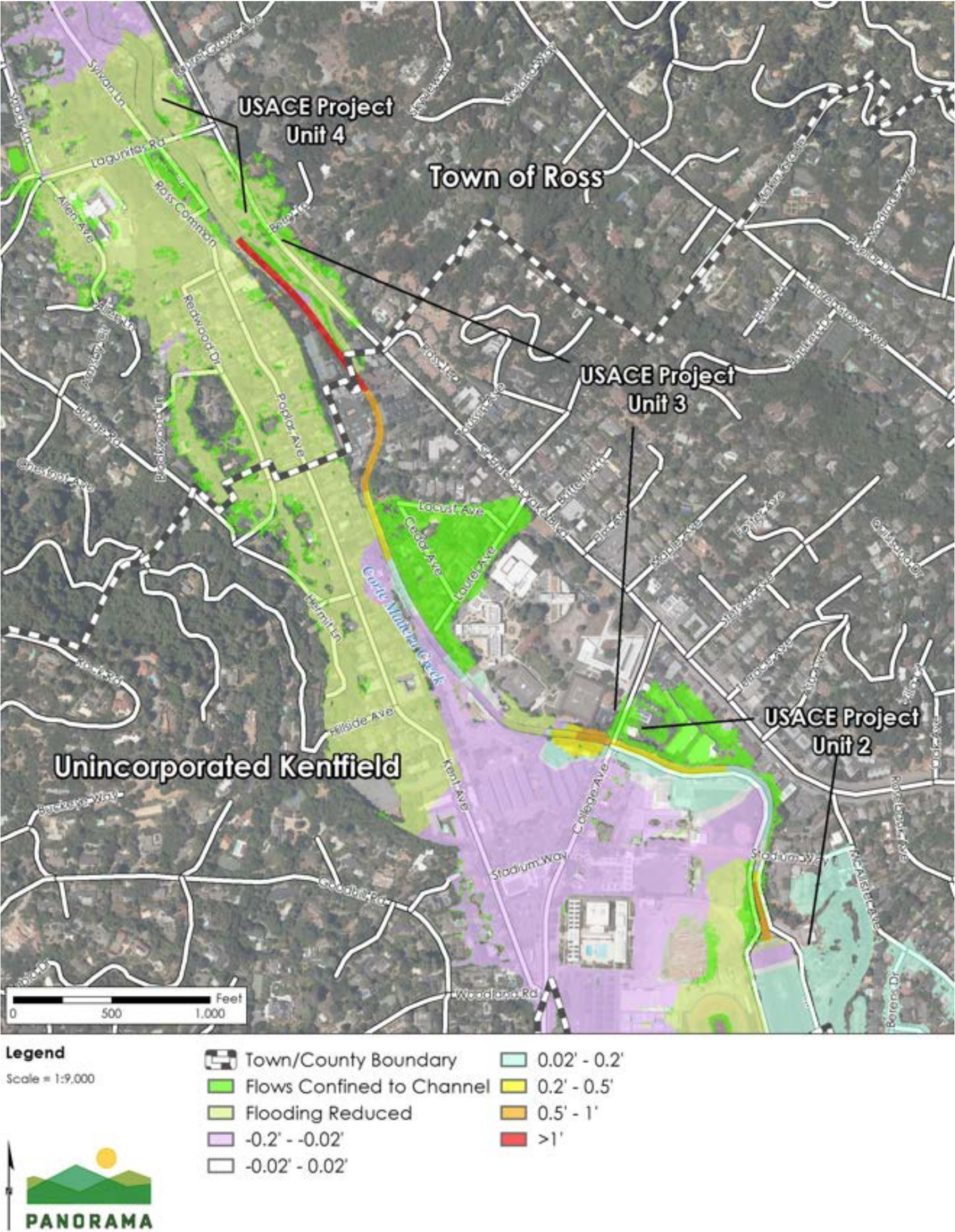
Figure 3.9-9 Project Changes in Water Surface Elevation from Future Conditions, 100-Year Flood Event
