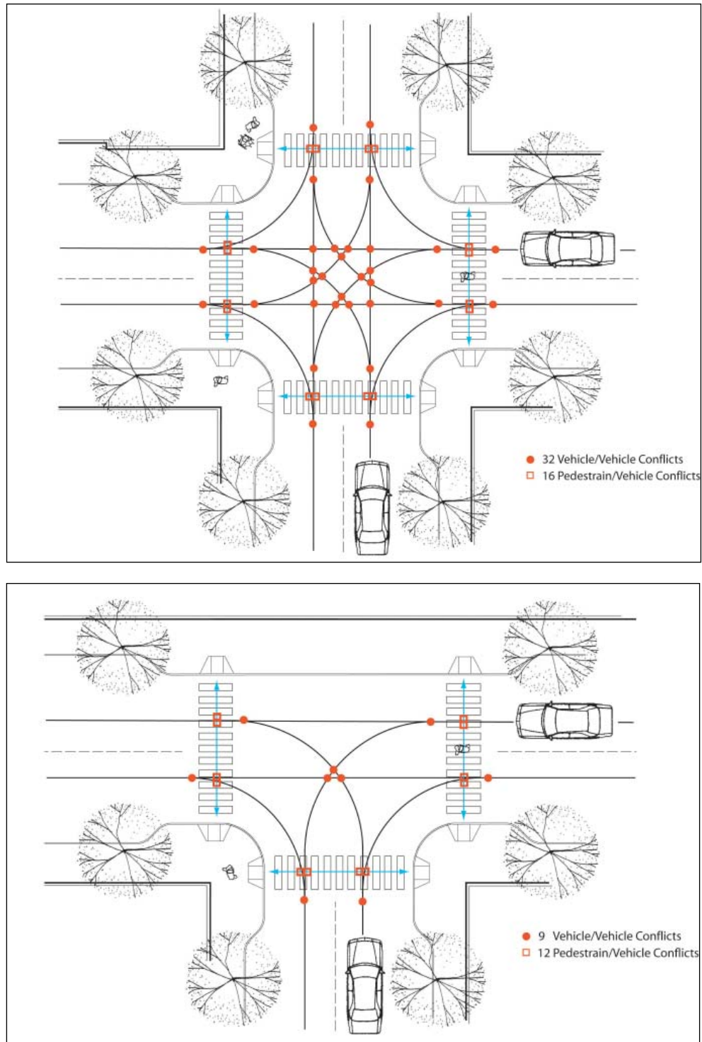
Figure 10.6 Vehicle and pedestrian conflicts at three- and four-leg intersection. Source: Community, Design + Architecture, adapted from an illustration by Michael Wallwork.
