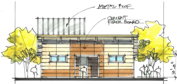
SOUTH ELEV
