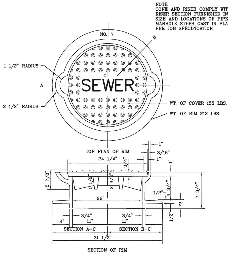
STANDARD MANHOLE RIM AND COVER
