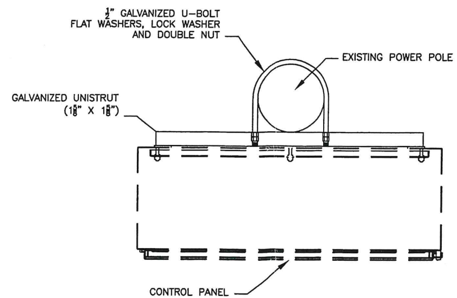
CONTROL PANEL MOUNTING DETAIL TOP PLAN
