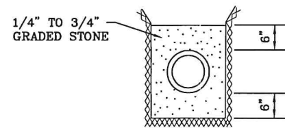
OVER 20' OF COVER
