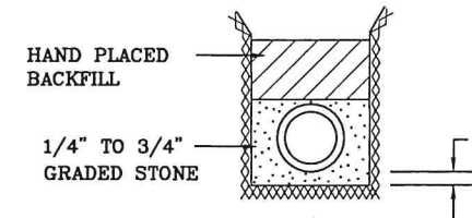
3' TO 20' OF COVER
