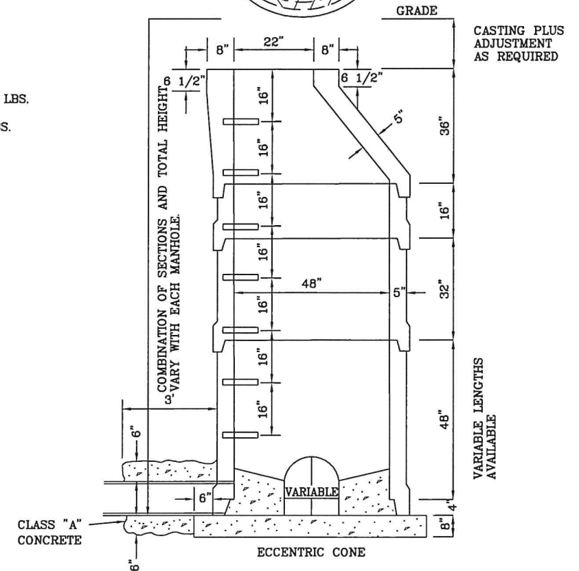
48" PRECAST CONCRETE MANHOLE
