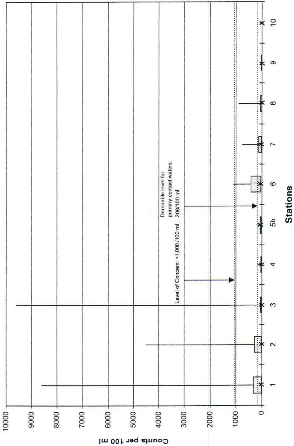
Figure 8 Fecal Coliform Counts for Selected Streams Sites in the Upper Wolf Creek Watershed
