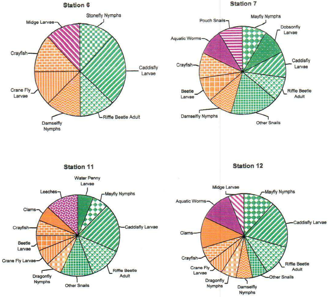
Figure 12 Composition of Selected Macroinvertebrate Groups for Four Stations in the Upper Wolf Creek Watershed
