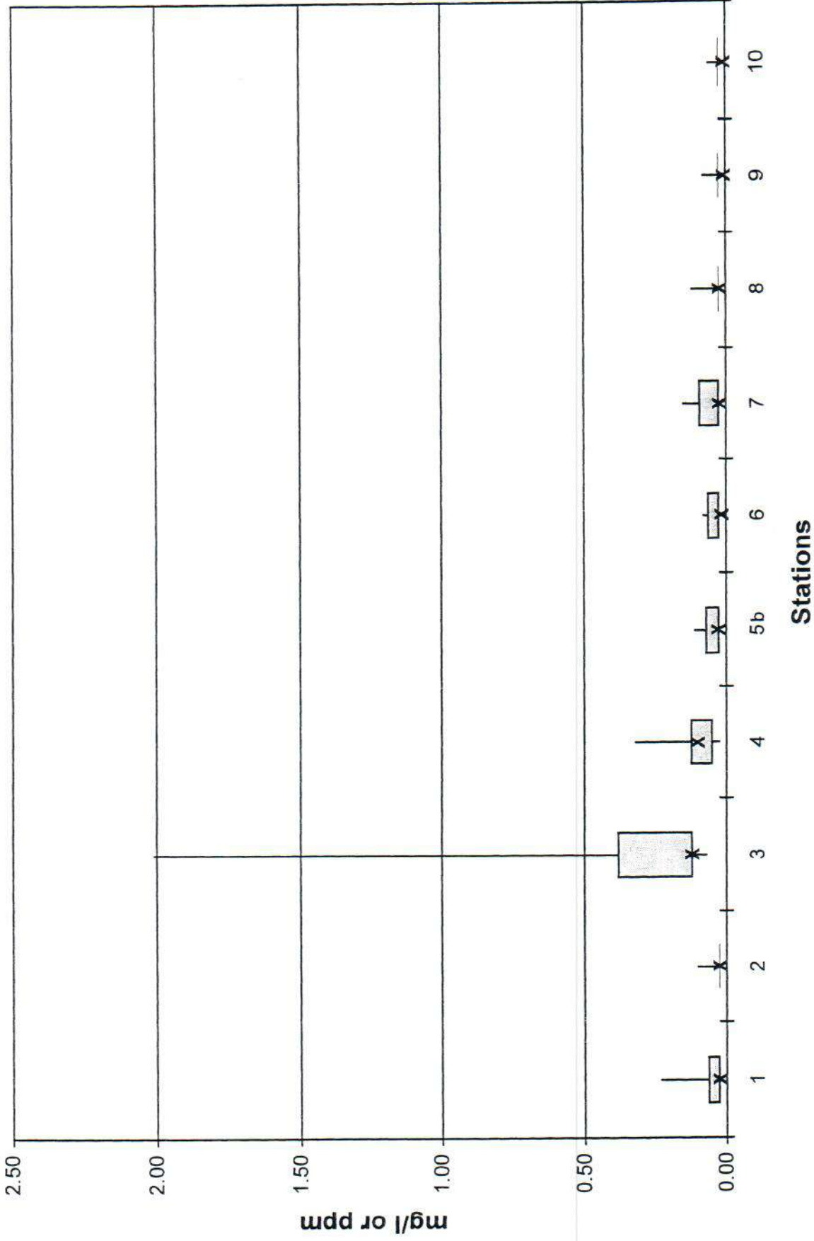
Figure 3 Concentrations of Ammonia for Selected Stream Areas in the Upper Wolf Creek Watershed
