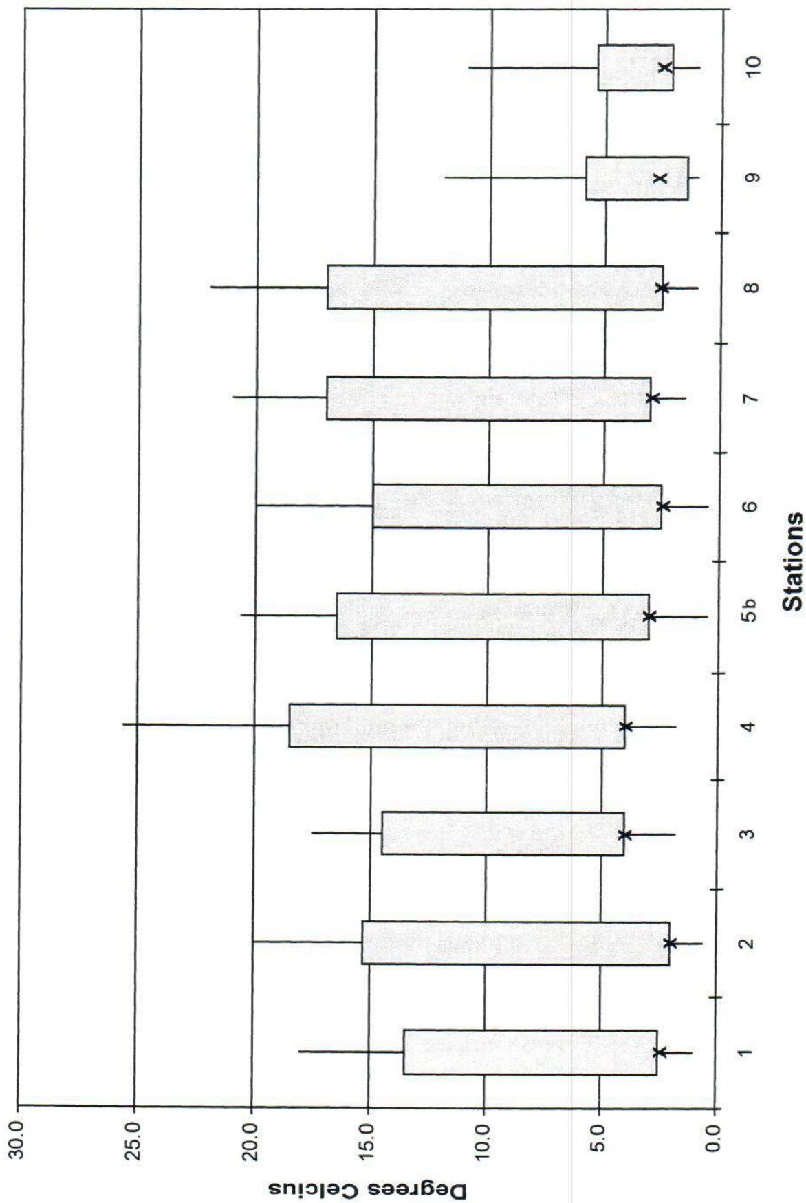
Figure 11 Temperatures for Selected Stream Areas in the Upper Wolf Creek Watershed
