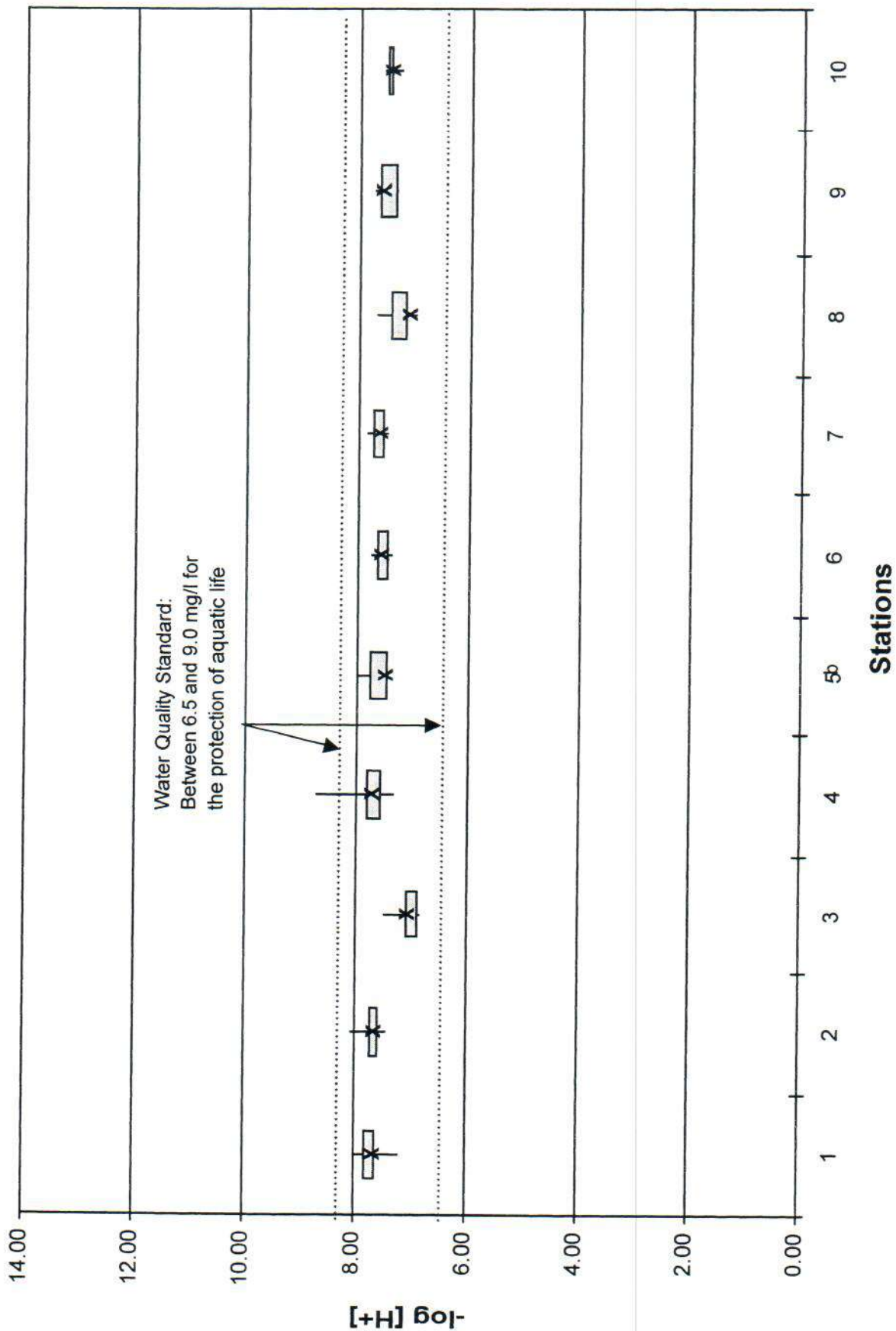
Figure 10 pH Levels for Selected Stream Locations in the Upper Wolf Creek Watershed
