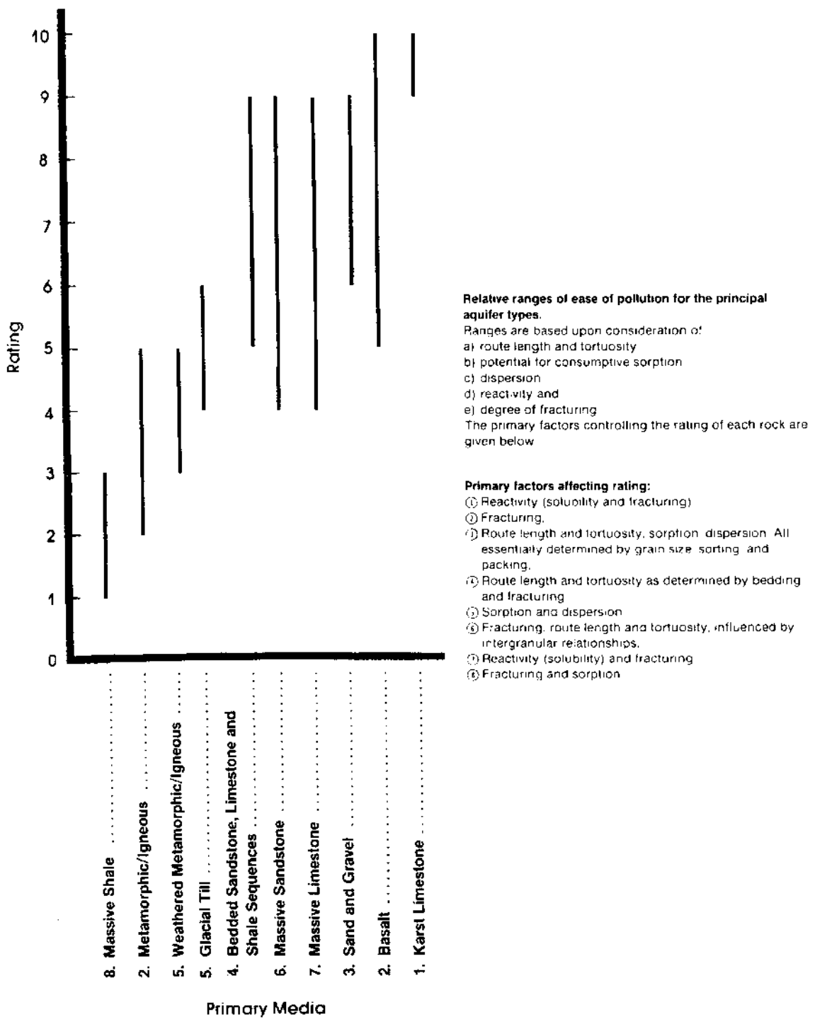
Figure 5. Graph of ranges and ratings for aquifer media.
