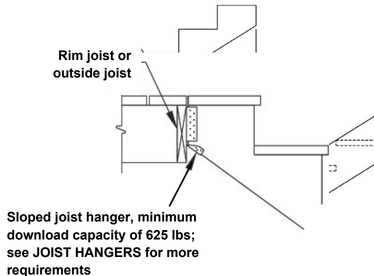
Figure 24. Stair Stringer Attachment Detail
