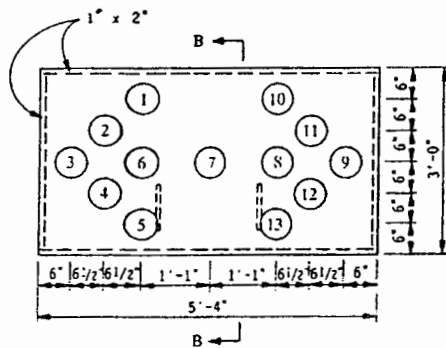
LIGHTED ARROW-TYPE B (FRONT PANEL-PAINTED FLAT BLACK)
