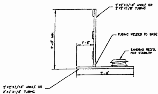
STEEL SUPPORTS
