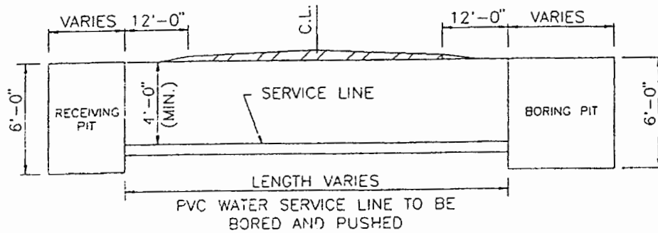
SECTION "A"
