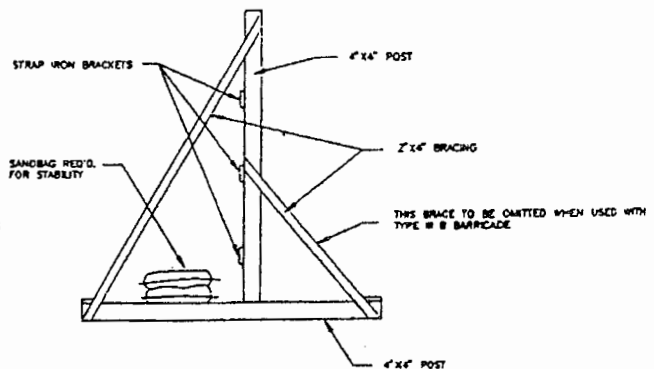
DETAIL OF TYPICAL SIGN STANDARD (T.S.S.)
