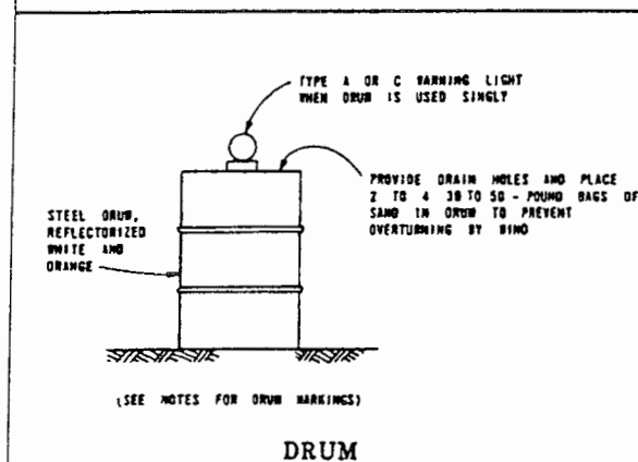
DRUM SYMBOLS
