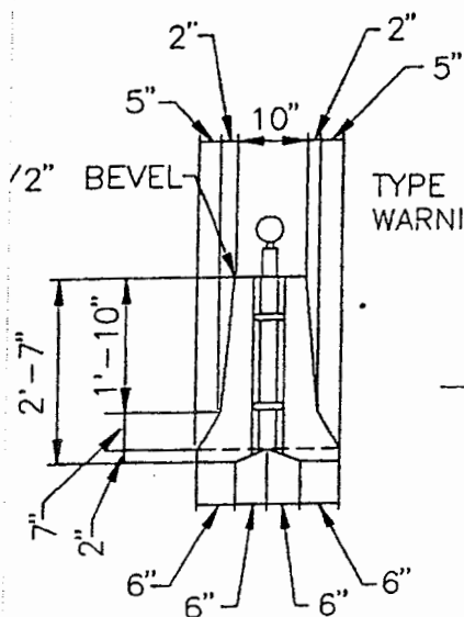
END VIEW NOT TO SCALE
