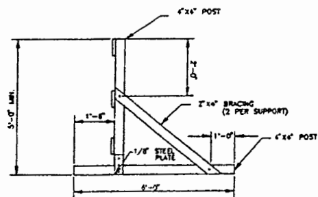
WOOD SUPPORTS
