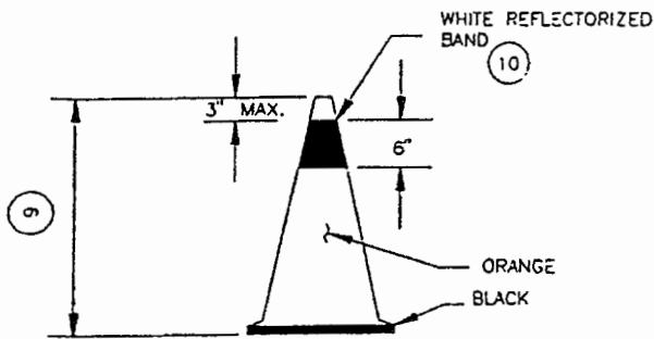
STANDARD CONE
