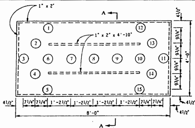
LIGHTED ARROW-TYPE A (FRONT PANEL-PAINTED FLAT BLACK)
