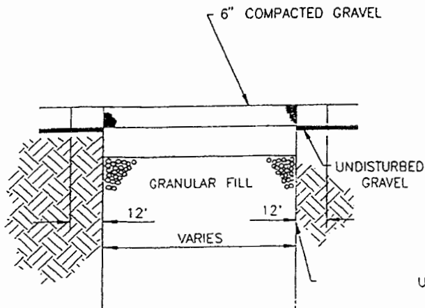
GRAVEL STREET REPAIR
