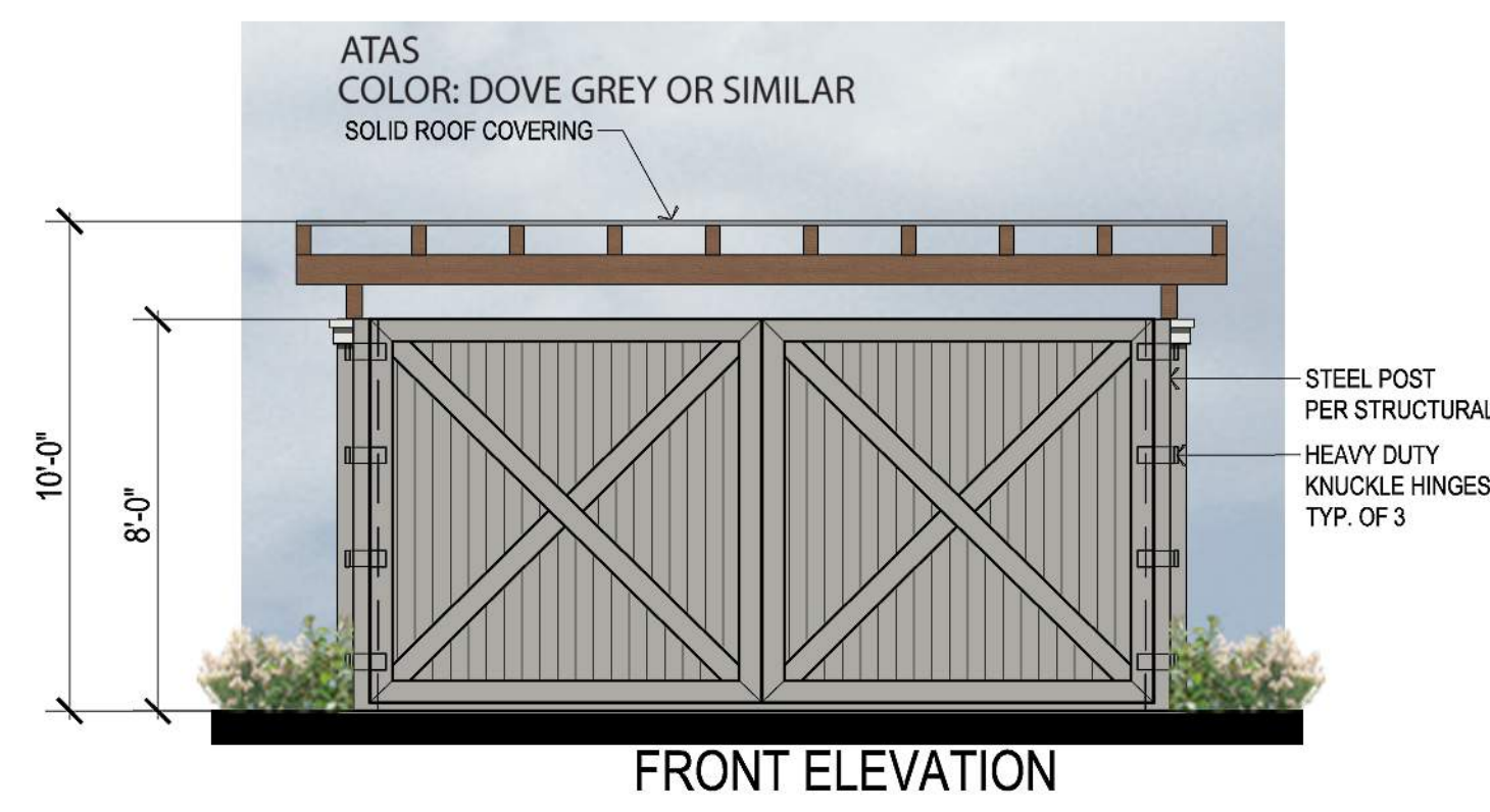
FRONT ELEVATION
