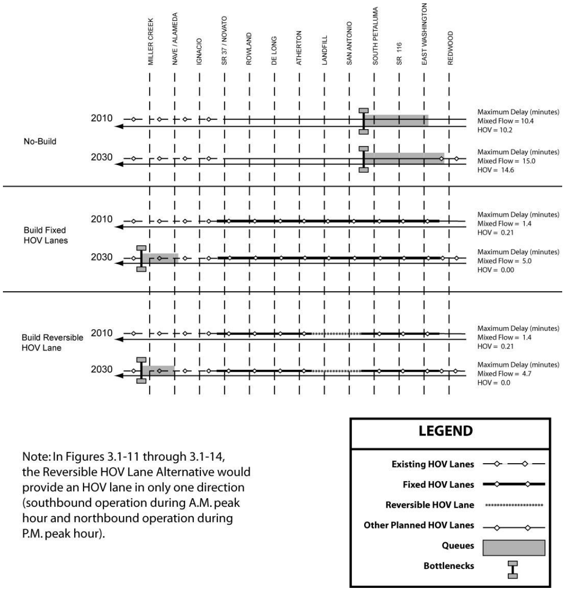
Figure 3.1-11 Southbound A.M. Peak Period—Expected Traffic Conditions
