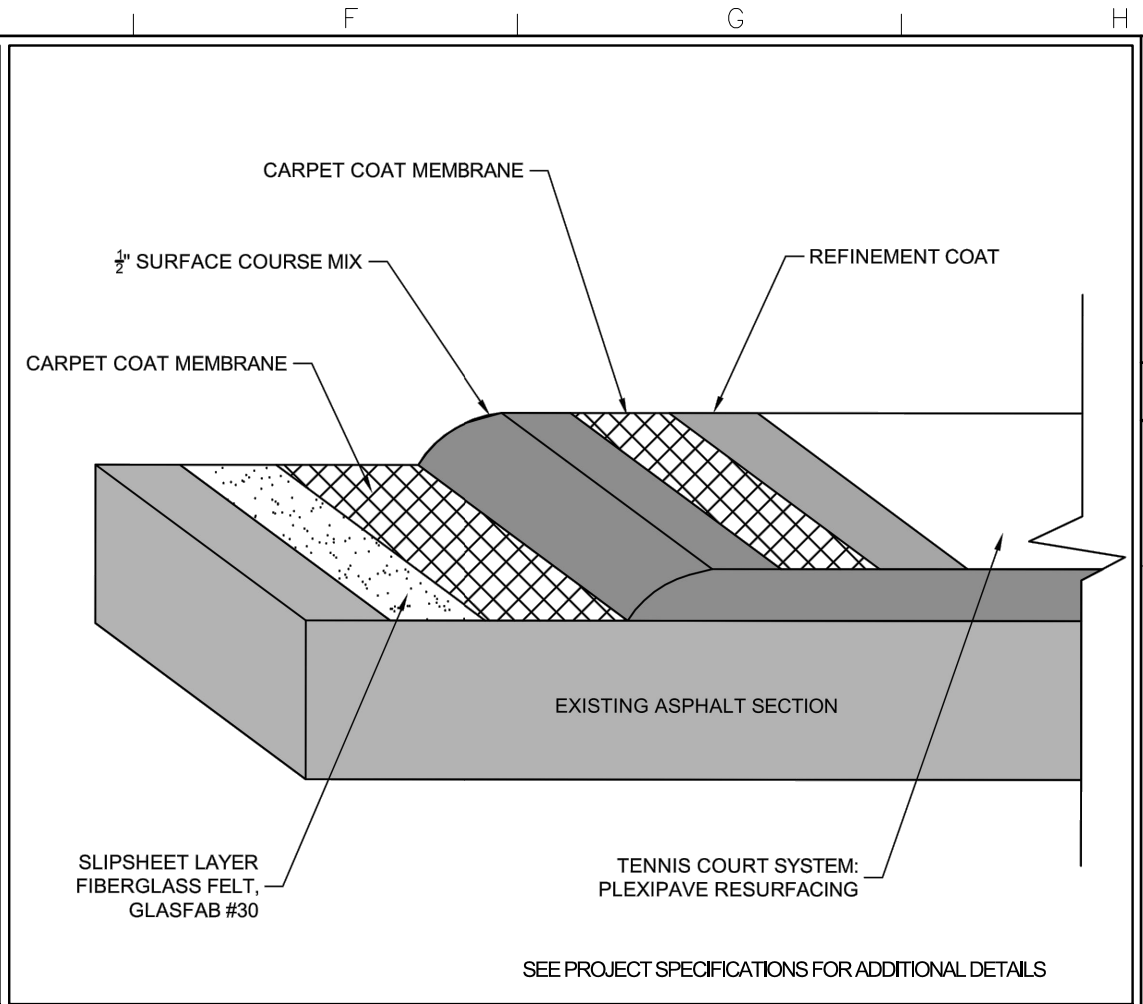
3 RESURFACE SECTION NO SCALE
