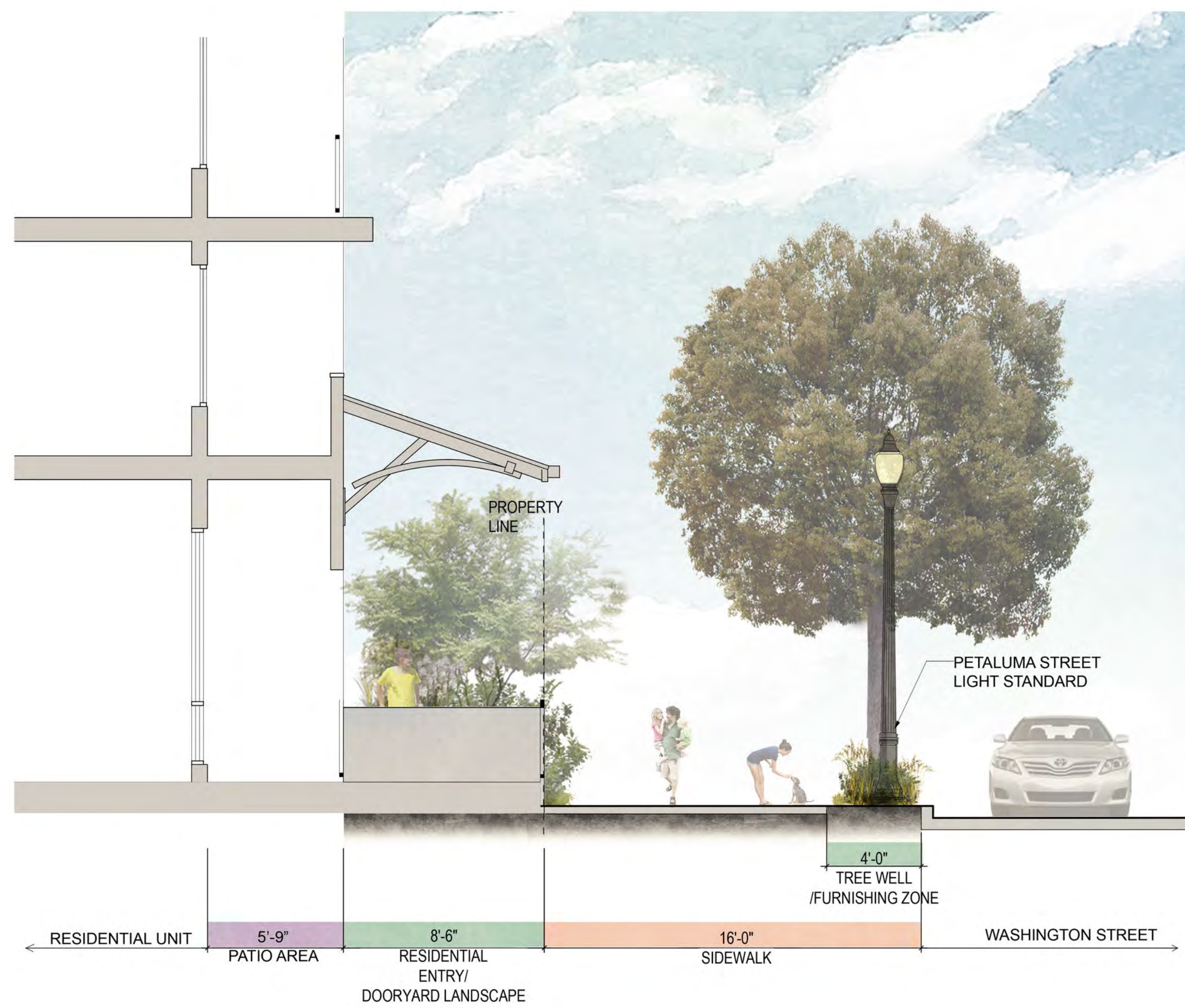
Section A-A' WASHINGTON STREET
