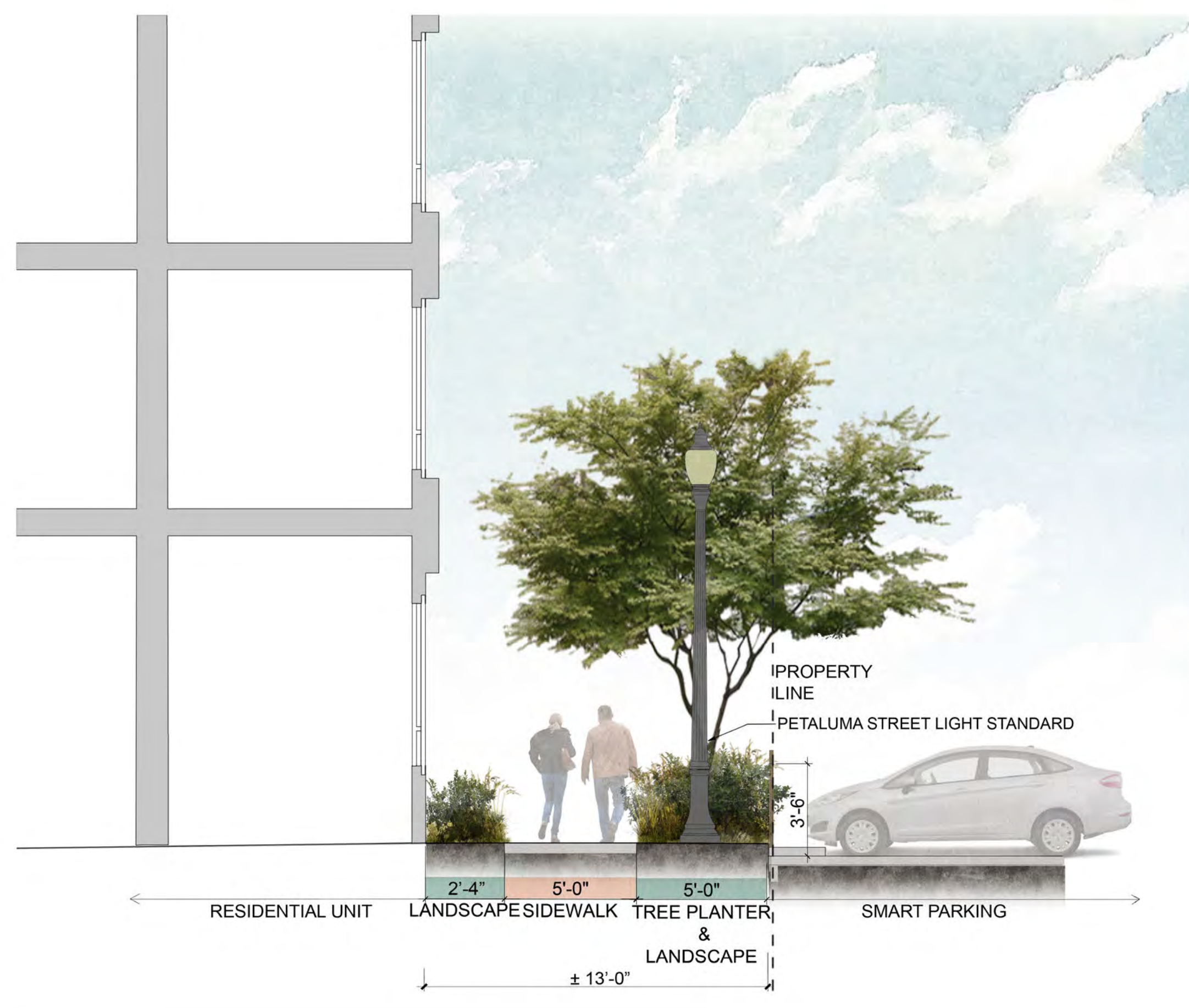
Section F-F' SMART STATION
