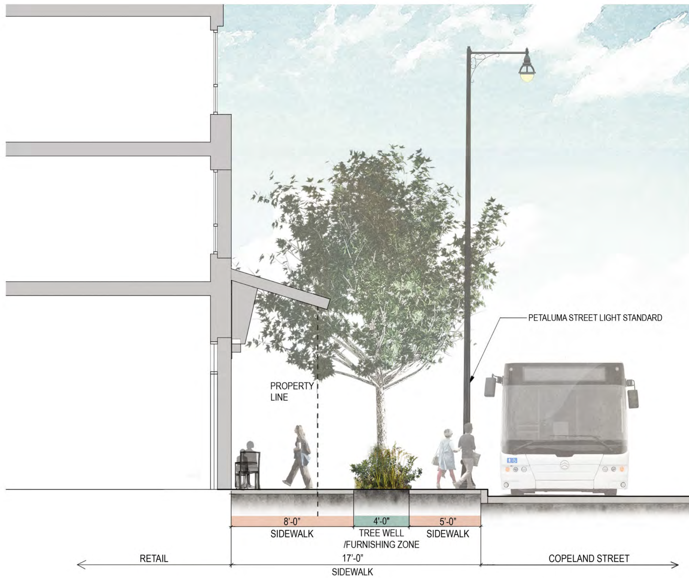
Section B-B' COPELAND STREET
