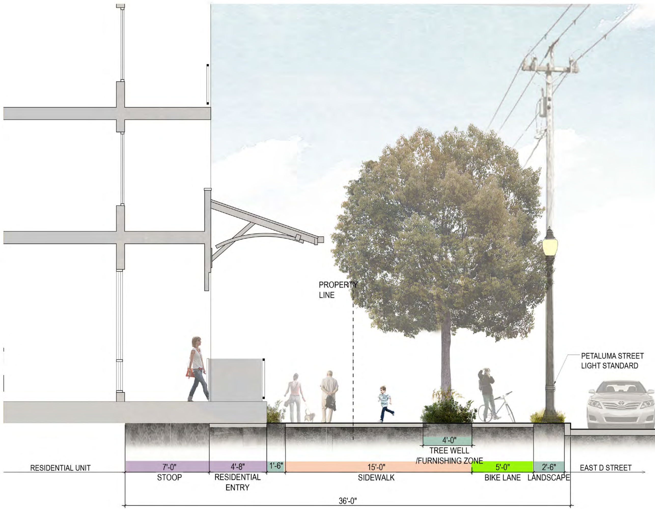
Section D-D' EAST D STREET
