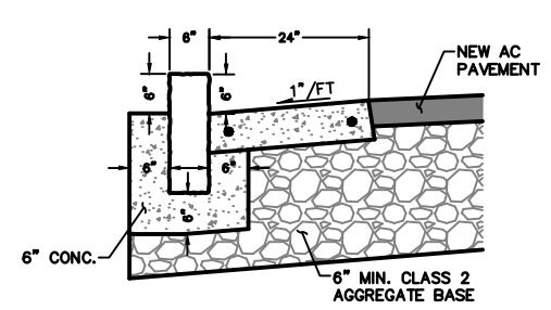
3 COBBLESTONE CURB & GUTTER SEE STD 216 FOR DETAILS NO SCALE
