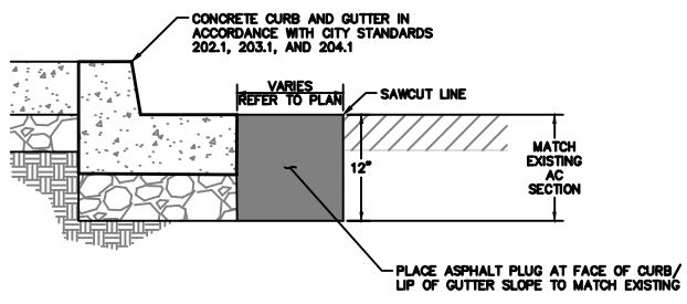
2 ASPAHLT CONCRETE PLUG NO SCALE
