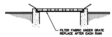
5 FILTER FABRIC NO SCALE
