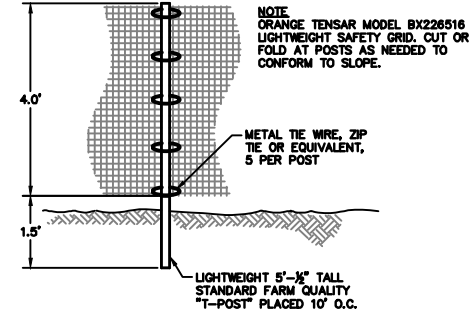
4 PROTECTION FENCE NO SCALE
