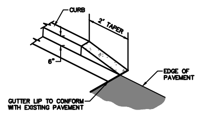
1 CURB TAPER NO SCALE
