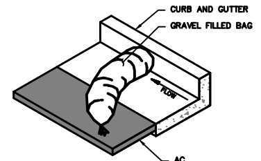
6 GRAVEL BAGS NO SCALE
