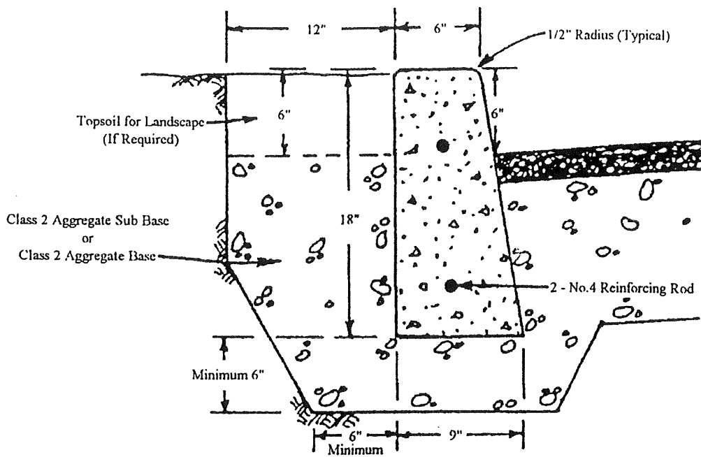
VERTICAL CURB
