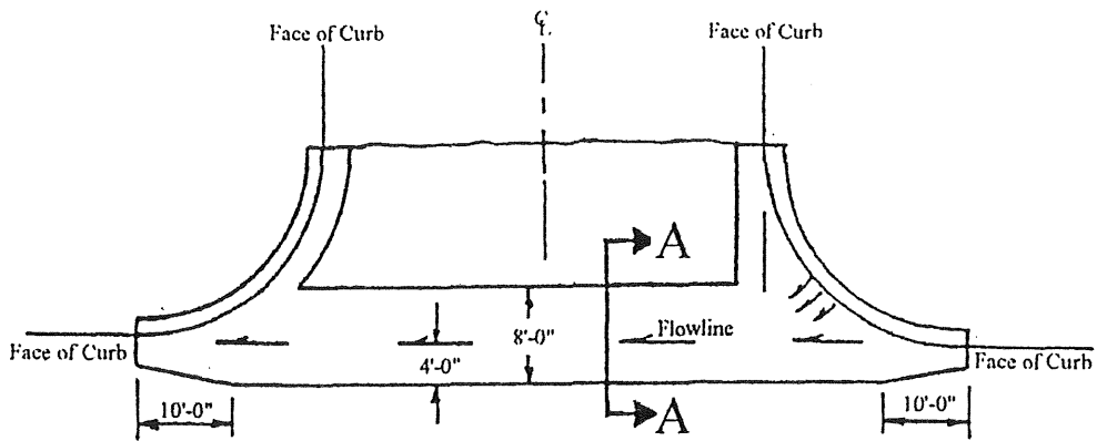
VALLEY GUTTER DETAIL
