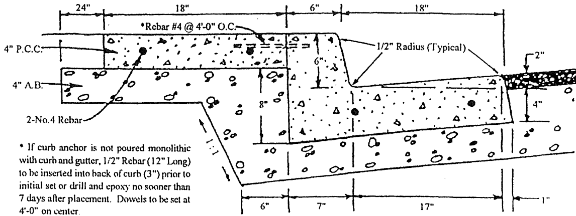
STANDARD CURB AND CUTTER with Curb Anchor
