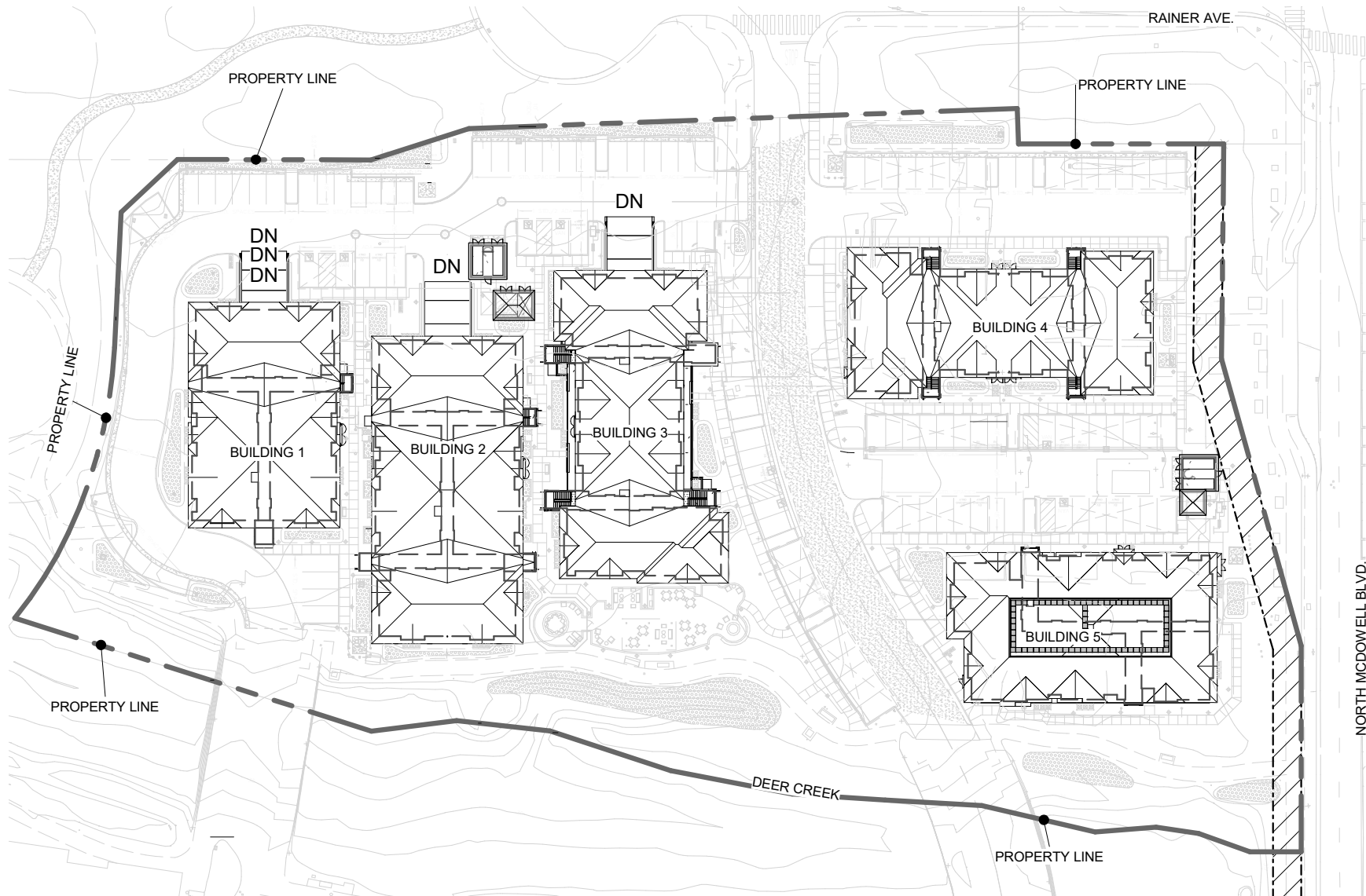
1 SITE PLAN 1" = 80'-0"
