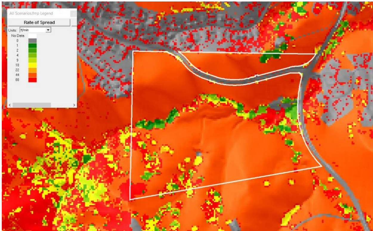
FIGURE 15 - PREDICTED RATE OF SPREAD (FEET/MINUTE) FOR THE NORTHEAST WIND SCENARIO DESCRIBED IN TABLE 8B.
