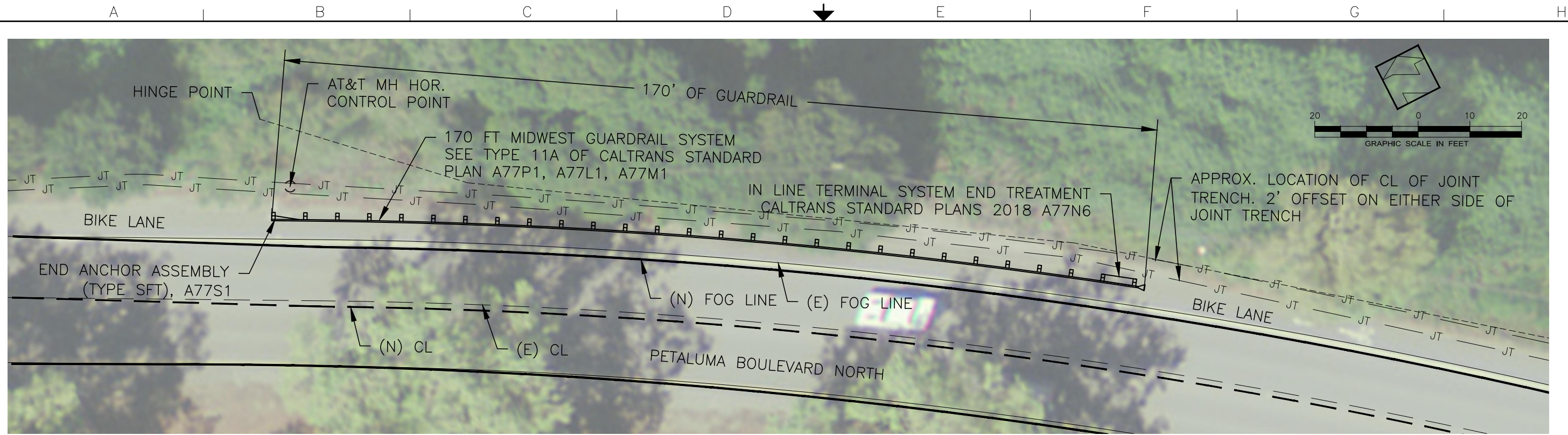
GUARDRAIL LAYOUT SCALE 1"=20"
