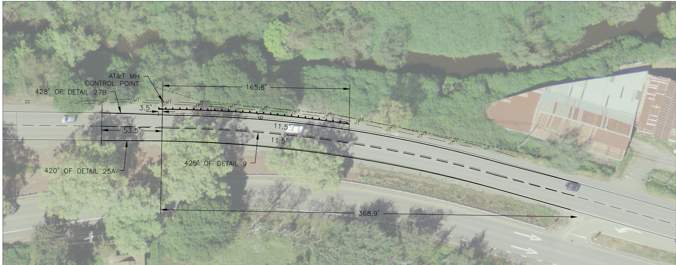
STRIPING LAYOUT AND HORIZONTAL CONTROL SCALE 1"=40'
