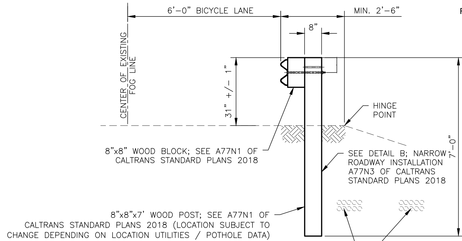
GUARDRAIL CROSS SECTION SCALE NTS
