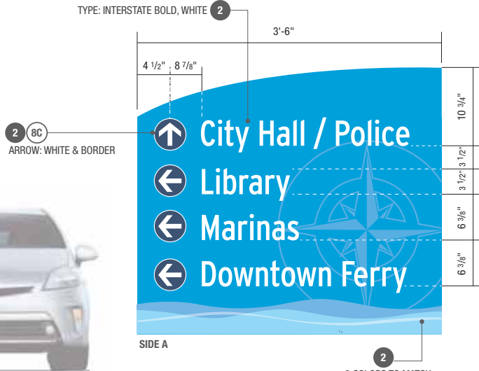
4 Detail Panel Layout / Vehicular Directional 1" = 1'-0"
