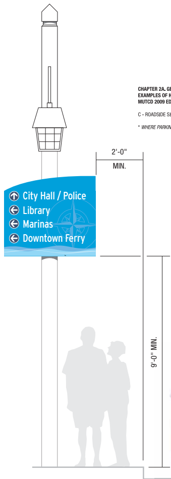
1 ELEVATION / Vehicular Directional 3/8" = 1'-0"
