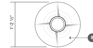
3 Partial Plan / Pedestrian Wayfinding / Directional 1" = 1'-0"
