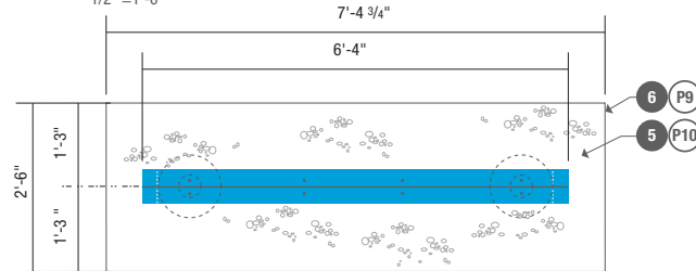
4 PLAN - Destination Sign / Small 1/2" = 1'-0"
