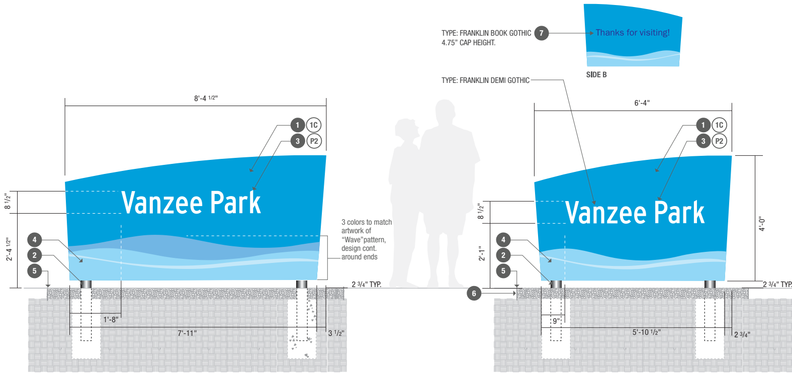
1 ELEVATION - Destination Sign / Large 1/2" = 1'-0"
