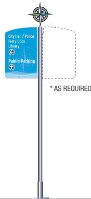
Pedestrian Wayfinding / Directional 1/4" = 1'-0" * AS REQUIRED
