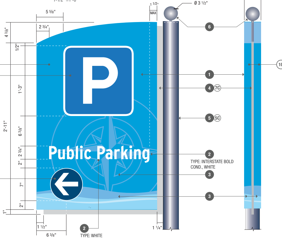
2 PLAN - Parking Directional / Parking ID 1-1/2" = 1'-0"
