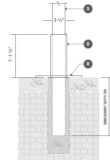
4 Detail / Pedestrian Wayfinding / Directional 1" = 1'-0"
