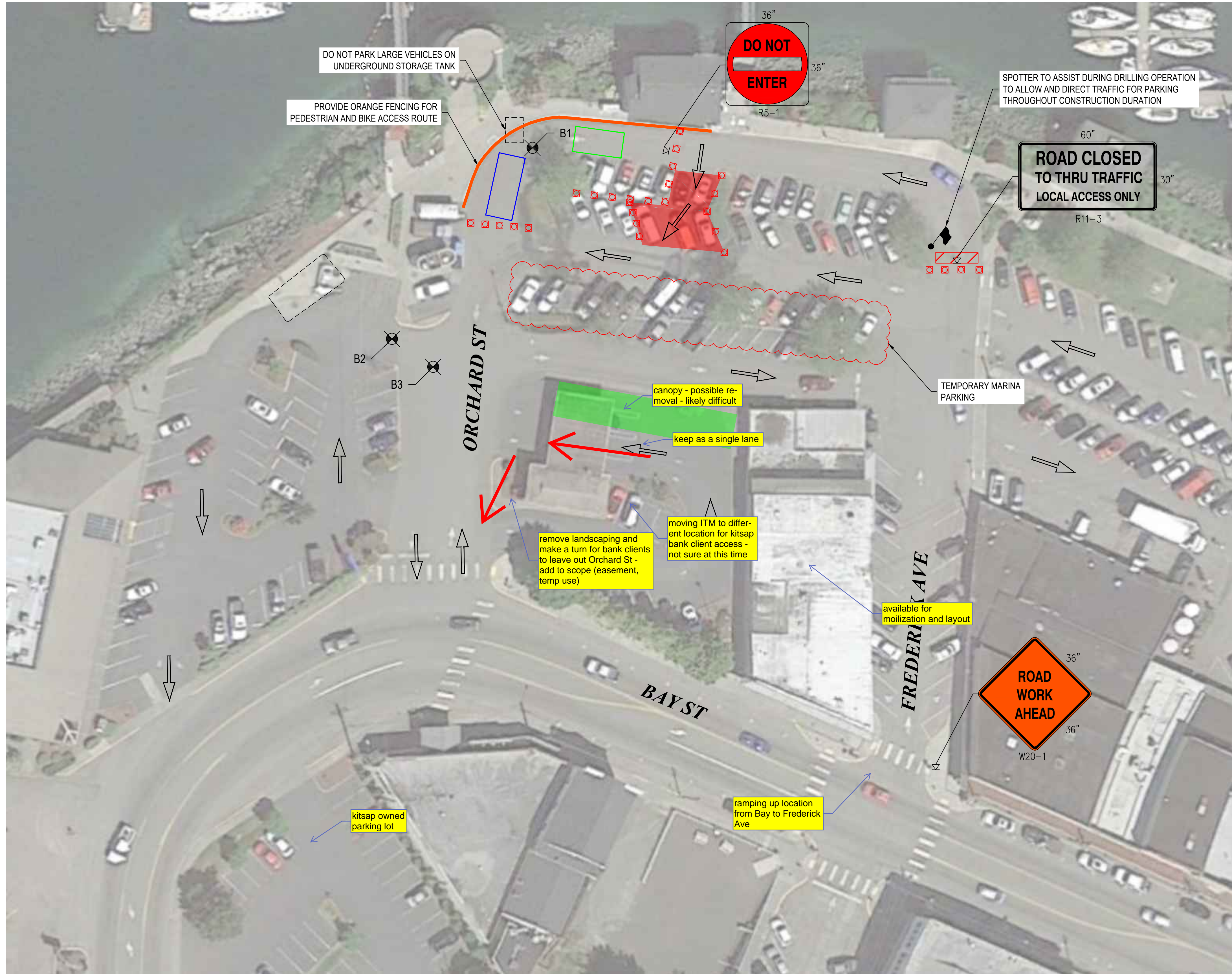
TRAFFIC CONTROL PLAN 1" = 30'
