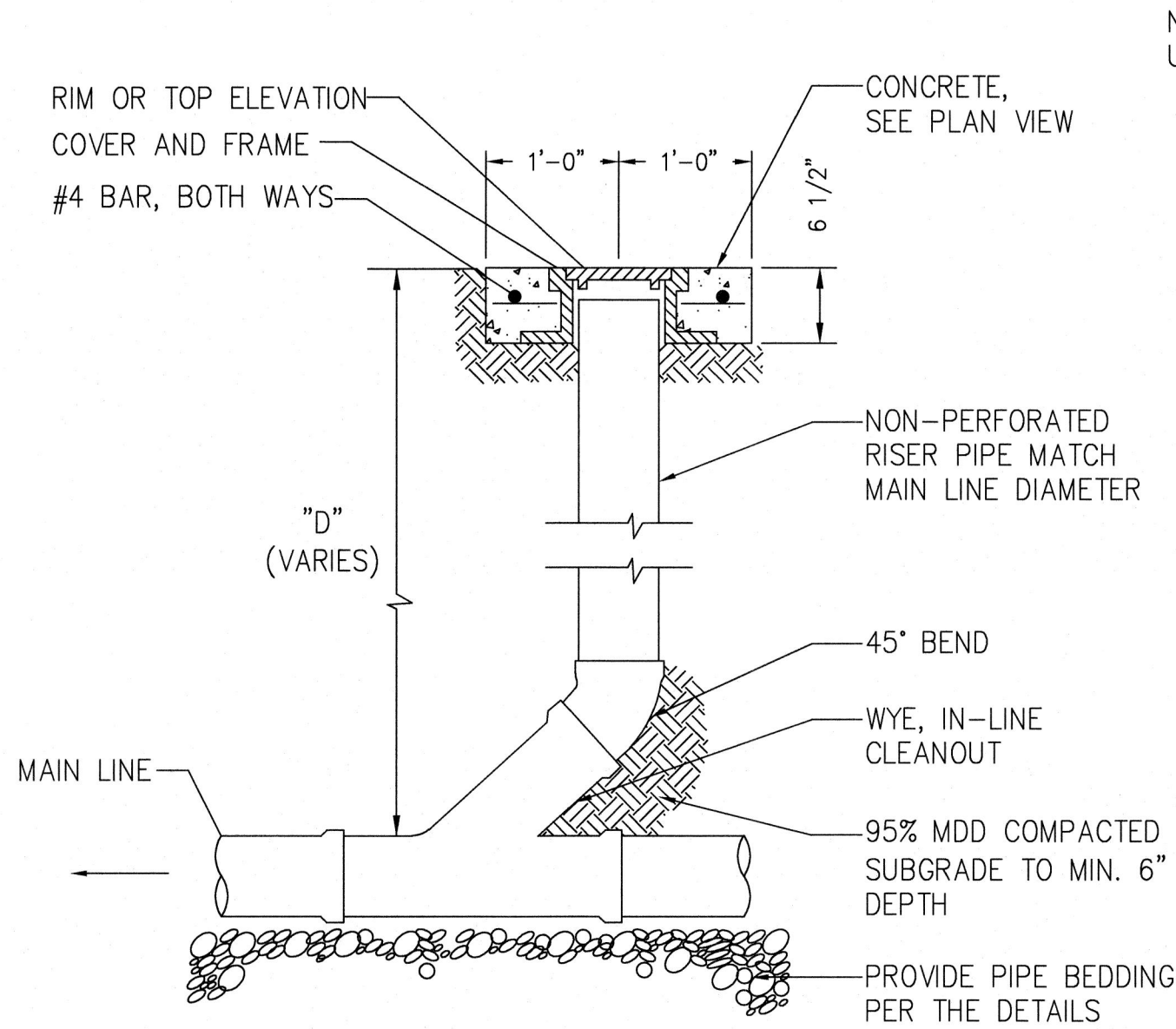
STORM DRAIN CLEANOUT NOT TO SCALE
