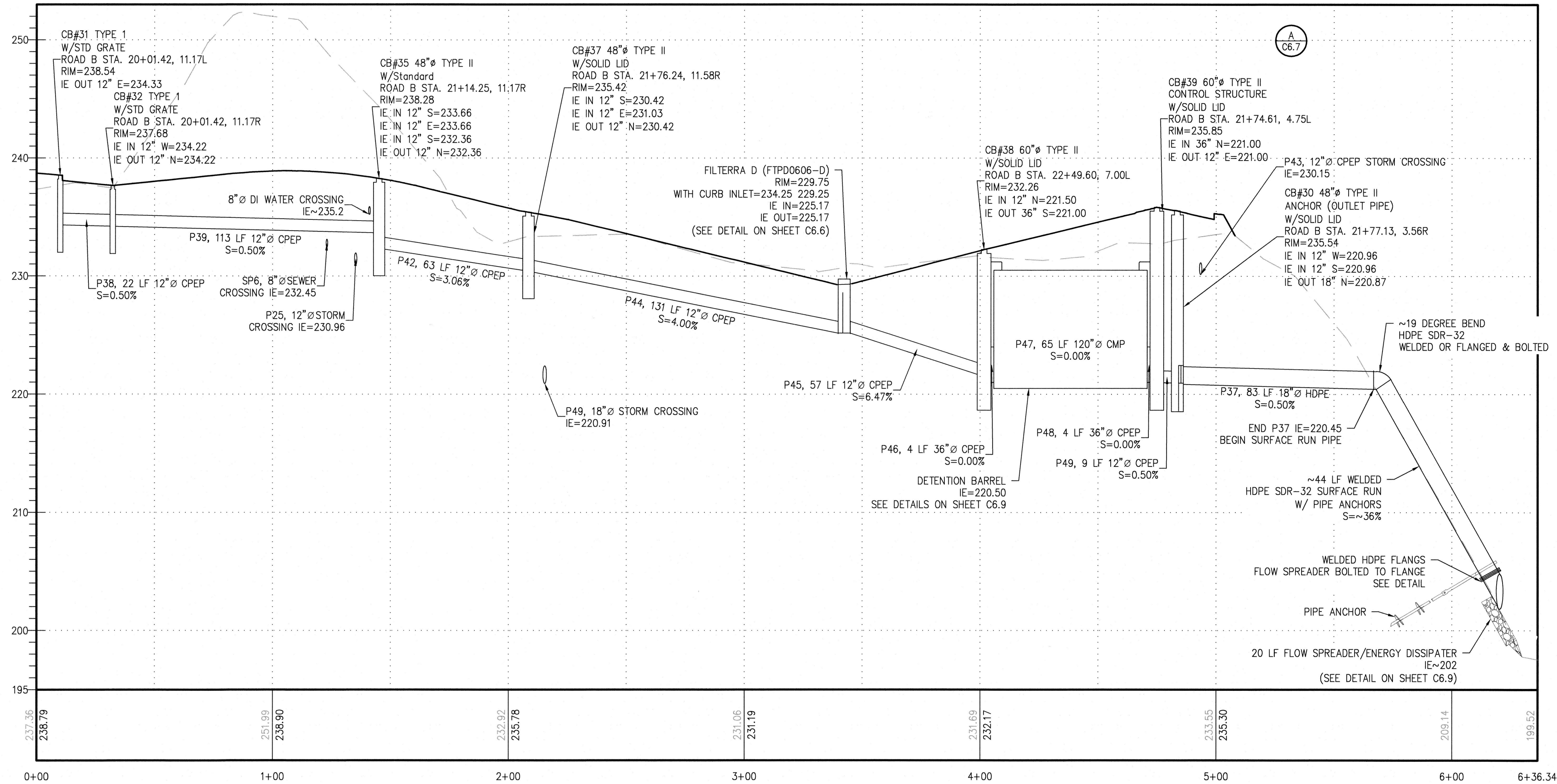
CB#31 TO OUTLET SCALE HORIZ: 1"=30' VERT: 1"=6'
