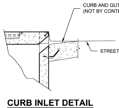
CURB INLET DETAIL
