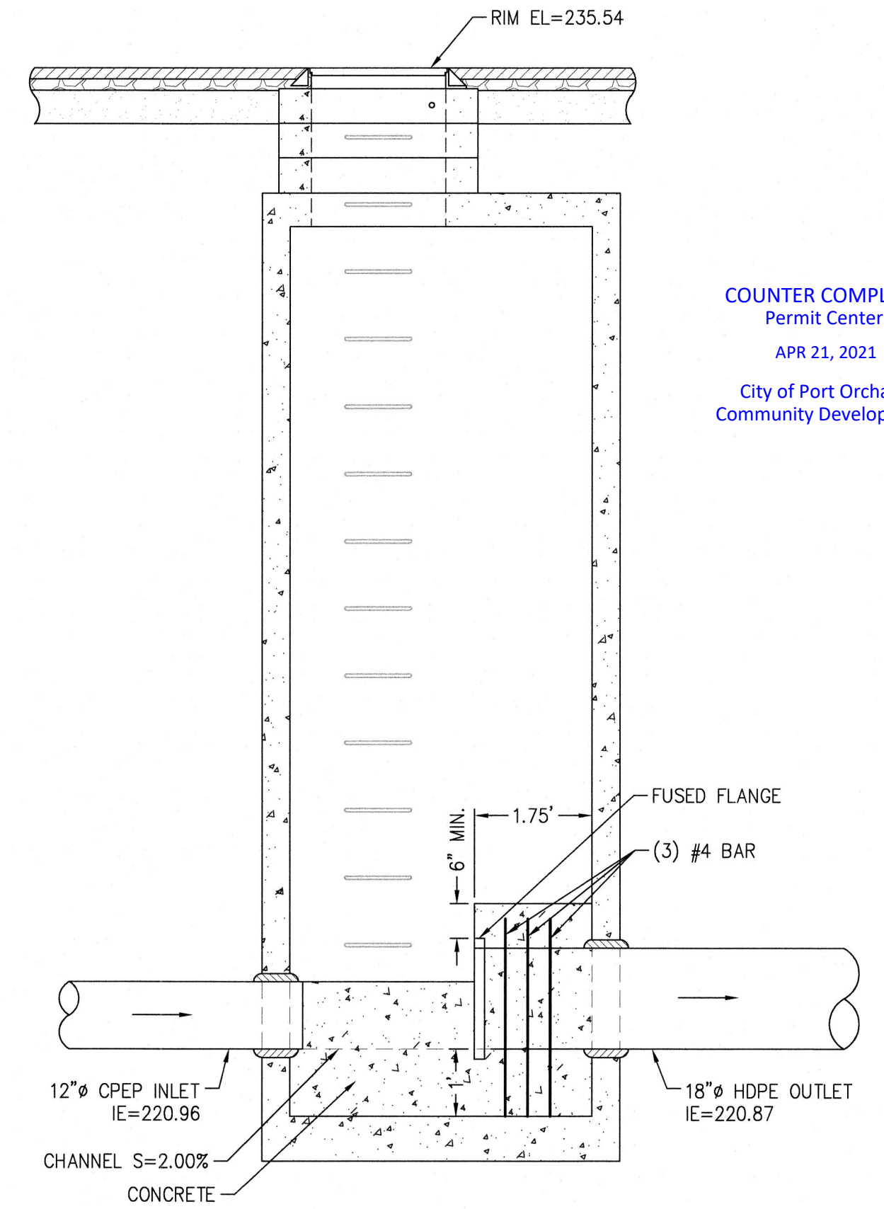
CB#30 54" ANCHOR CB SCALE 1"=2'
