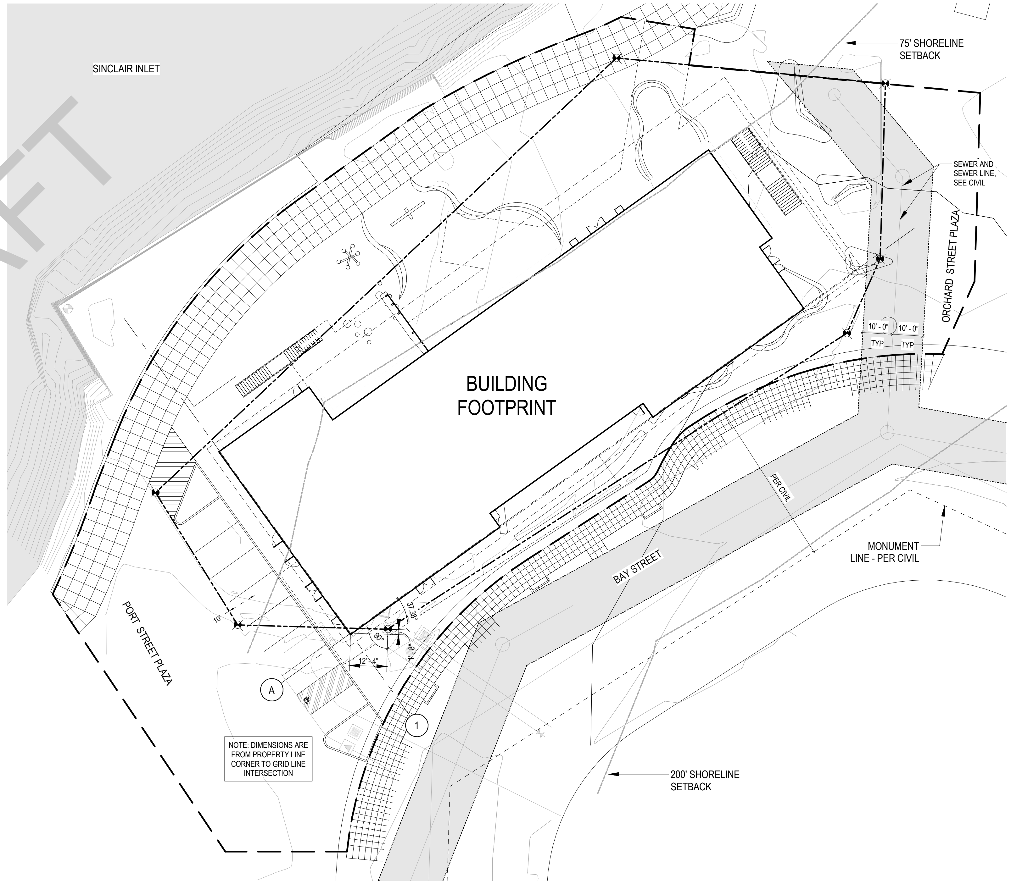
1 SITE PLAN 1" = 20'-0"
