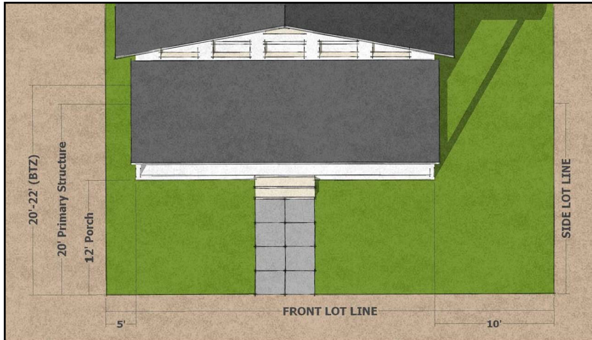
Figure 2 - Primary Structure Setbacks
