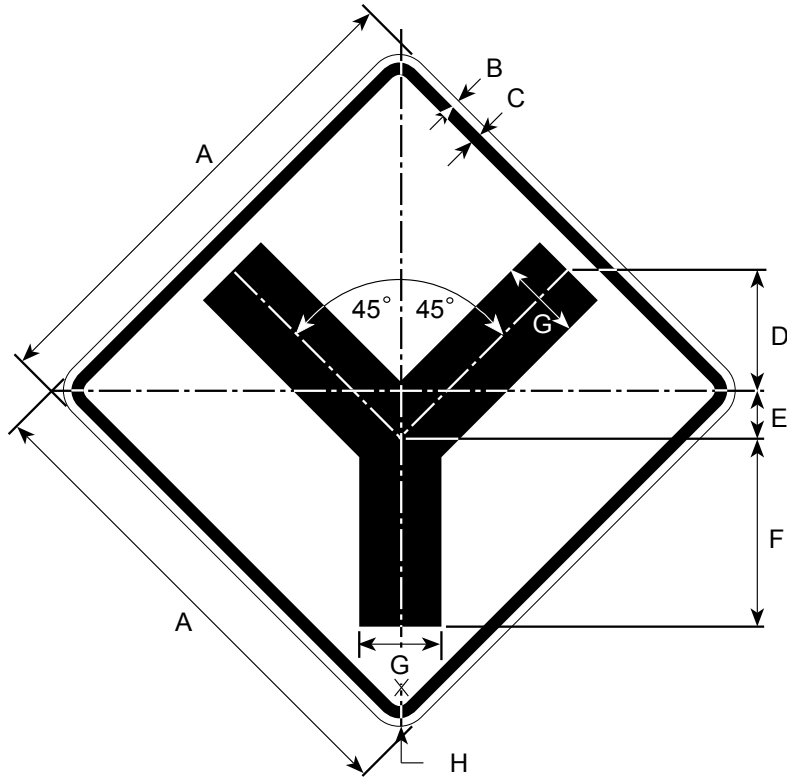
DIMENSIONS (MILLIMETERS)
