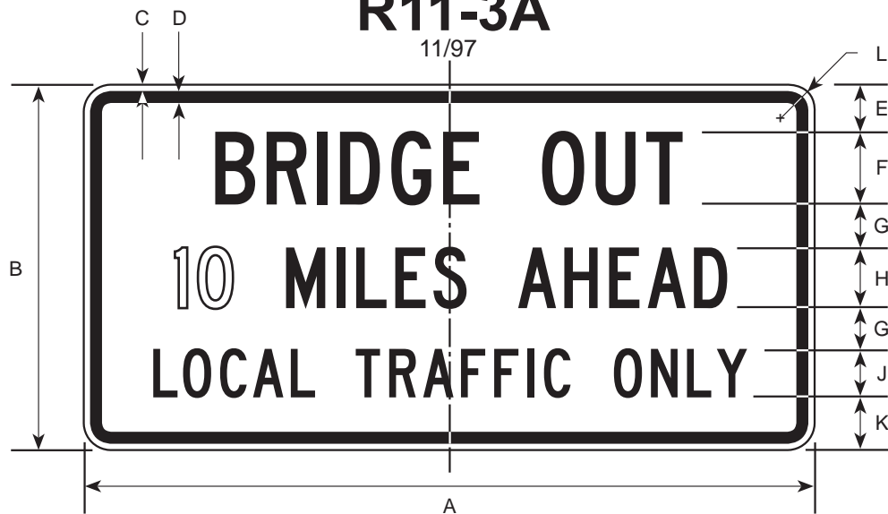
DIMENSIONS (MILLIMETERS)
