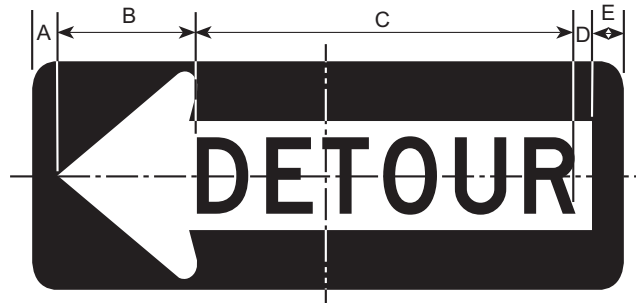
DIMENSIONS (MILLIMETERS)
