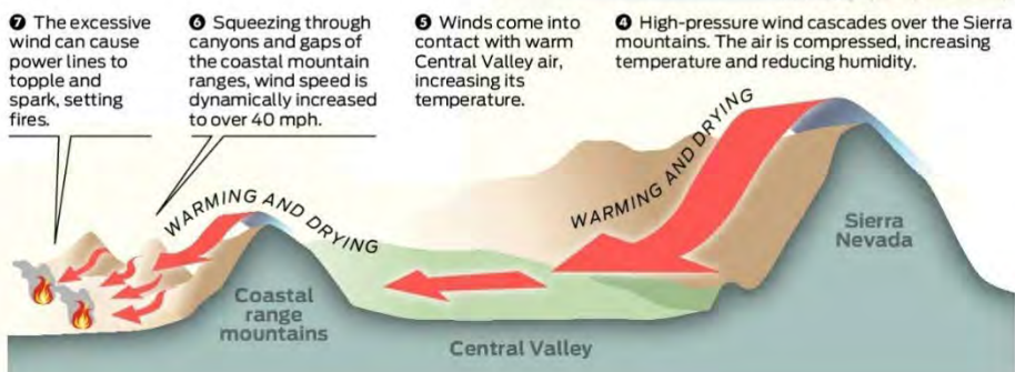
Figure 1.16: Diablo Wind Patterns
