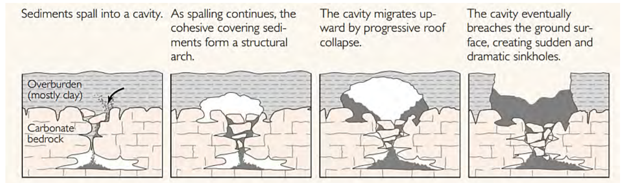
Figure 3.112: Cover-Collapse Sinkhole Formation Source: USGS
