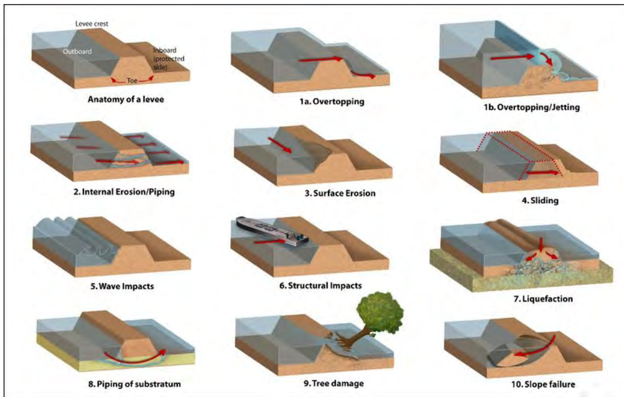
Figure 3.115: Levee Failure Mechanisms
