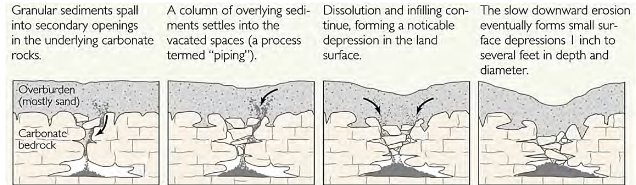
Figure 3.111: Cover-Subsidence Sinkhole Formation Source: USGS
