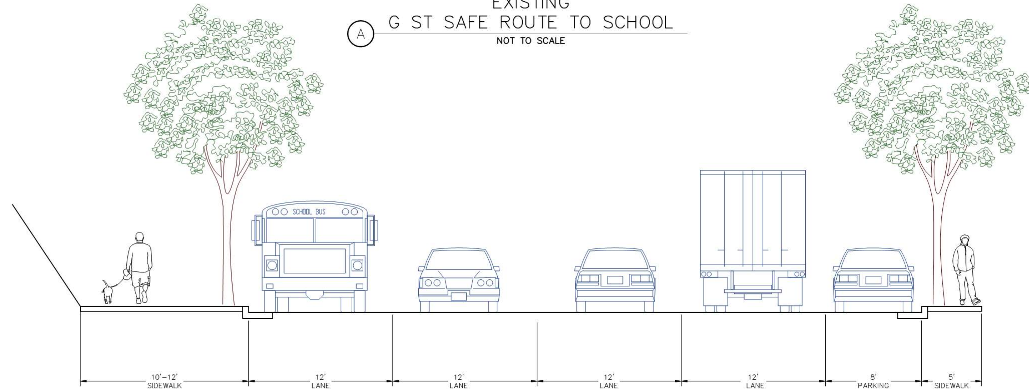
PROPOSED G ST SAFE ROUTE TO SCHOOL NOT TO SCALE
