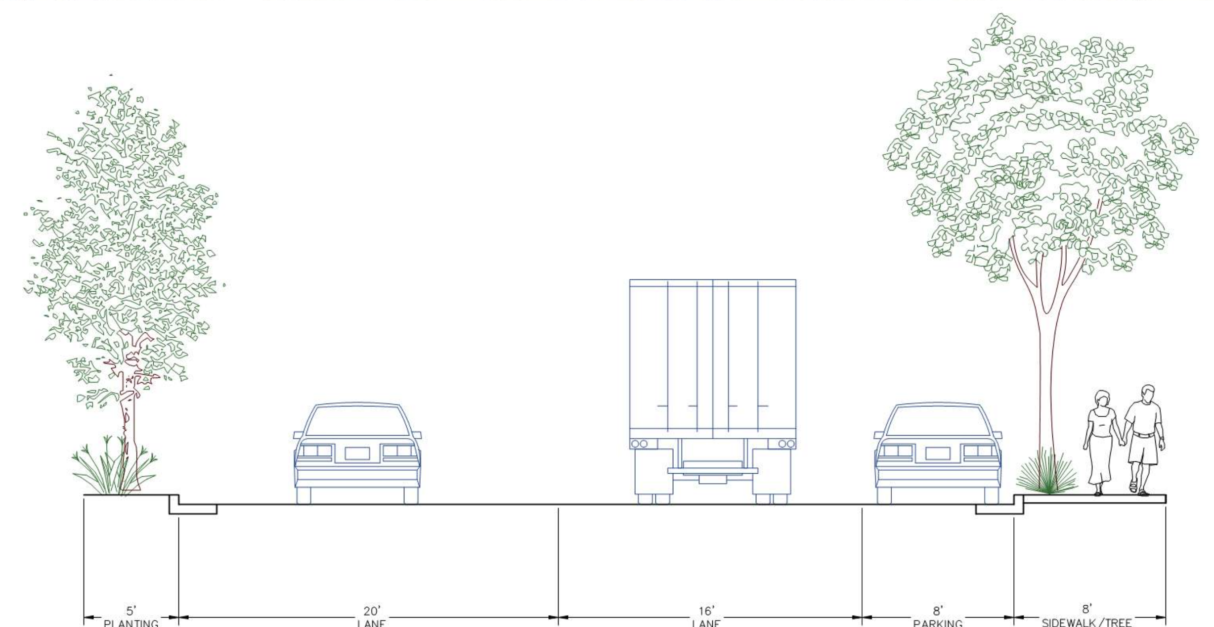
EXISTING HAYES ST TO SHAVER ST NOT TO SCALE
