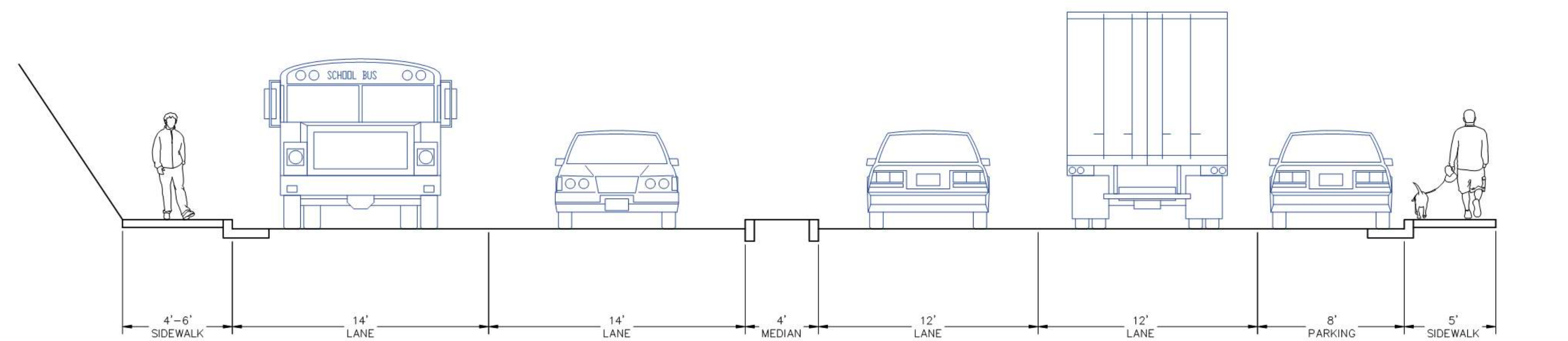
EXISTING G ST SAFE ROUTE TO SCHOOL NOT TO SCALE
