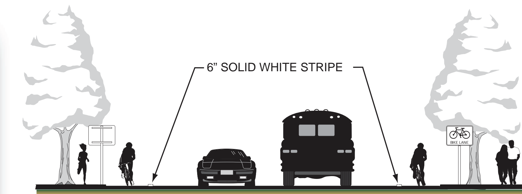
CLASS II BIKEWAY (Bike Lane) Provides a dedicated striped lane for one-way travel on a street or highway.
