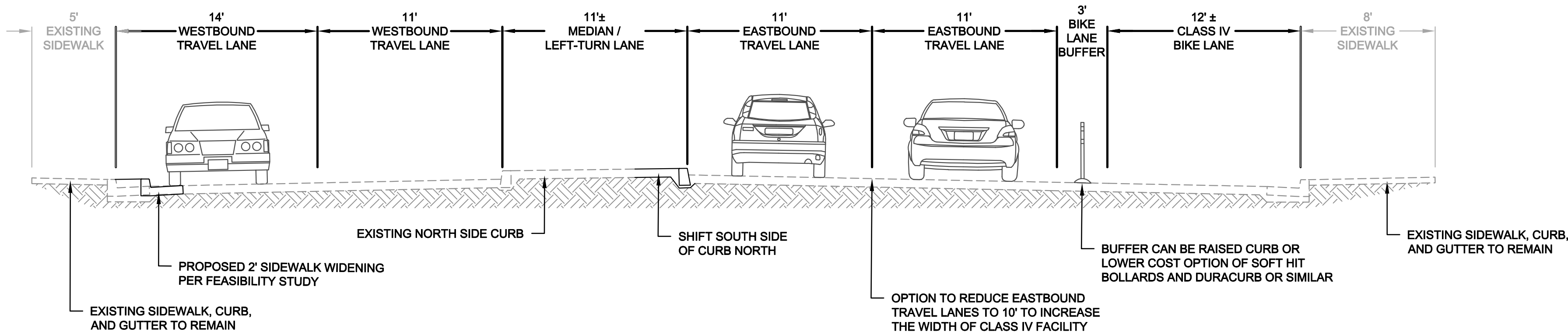
TYPICAL SECTION BETWEEN WEST AND EAST STREET
