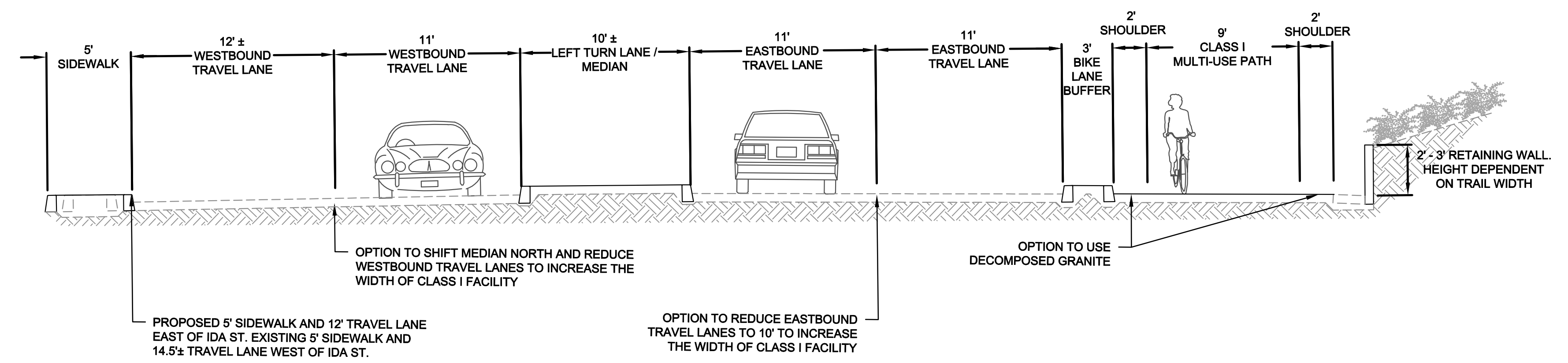
TYPICAL SECTION BETWEEN EAST AND G STREET
