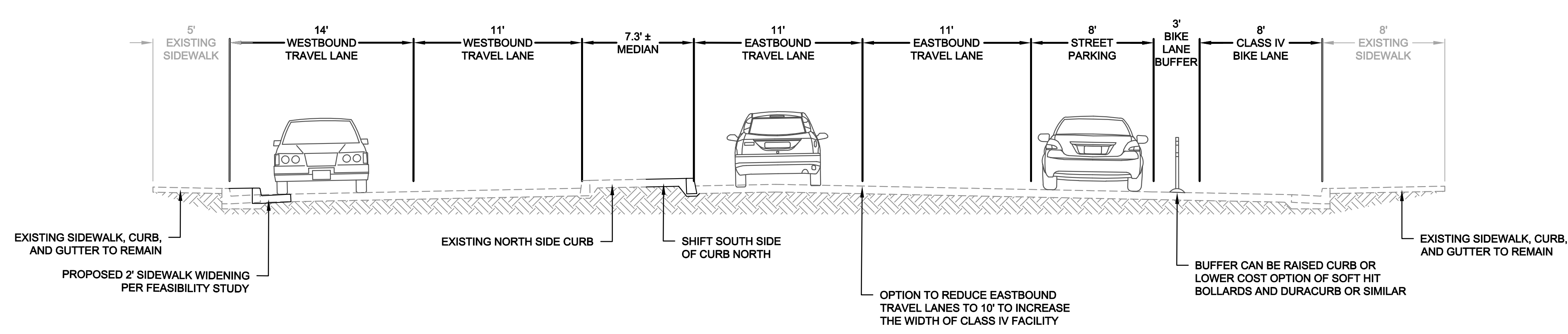
TYPICAL SECTION BETWEEN WEST AND EAST STREET
