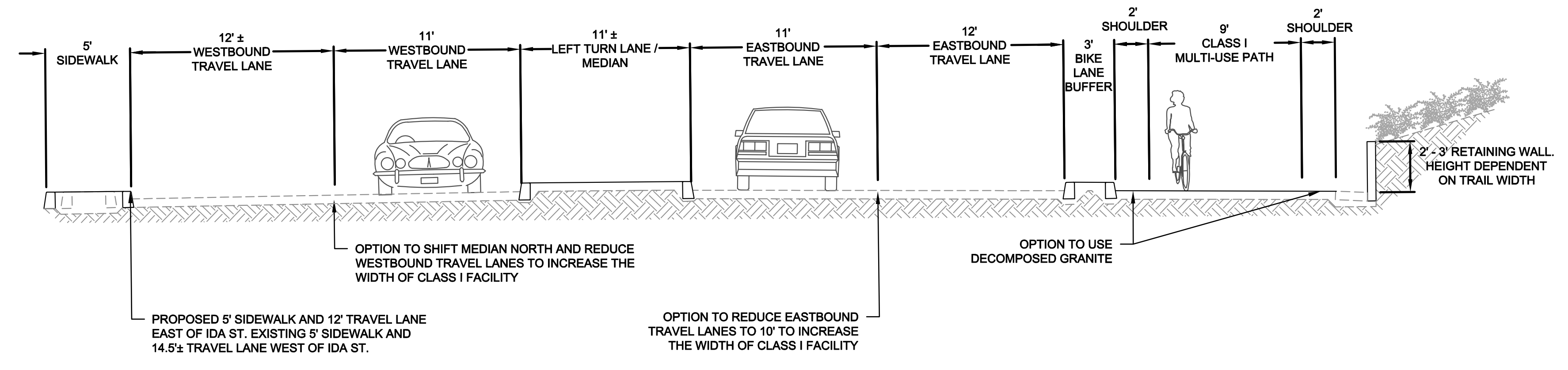
TYPICAL SECTION BETWEEN EAST AND G STREET
