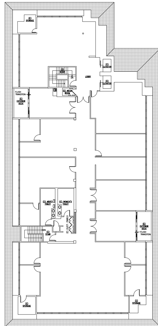
1 EXISTING THIRD FLOOR PLAN THIRD FLOOR AREA: 8,803 SF --- BUILDING FLOOR AREA: 24,042 SF (MEASURED TO INSIDE OF EXTERIOR WALLS, EXCLUDES STAIR ENCLOSURES AND ELEVATORS)
