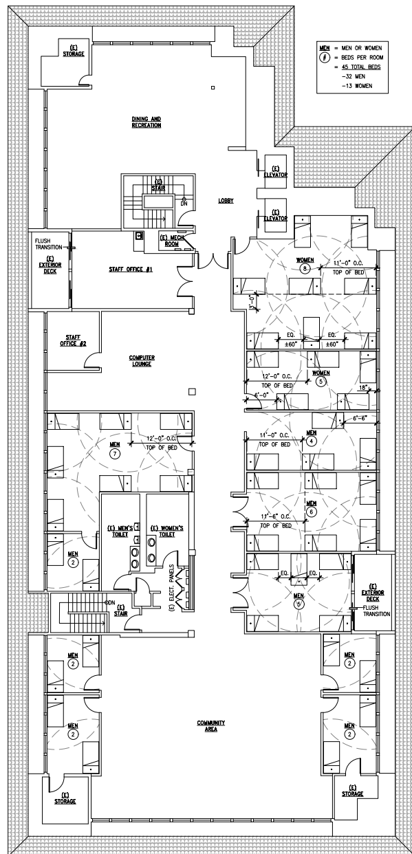
2 PROPOSED THIRD FLOOR PLAN THIRD FLOOR AREA: 8,803 SF --- BUILDING FLOOR AREA: 24,042 SF (MEASURED TO INSIDE OF EXTERIOR WALLS, EXCLUDES STAIR ENCLOSURES AND ELEVATORS)
