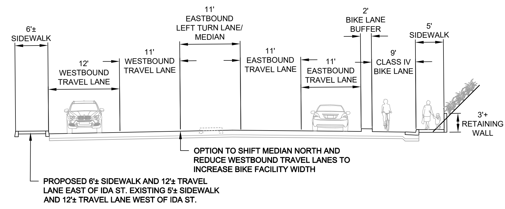
TYPICAL SECTION BETWEEN EAST AND G STREET
