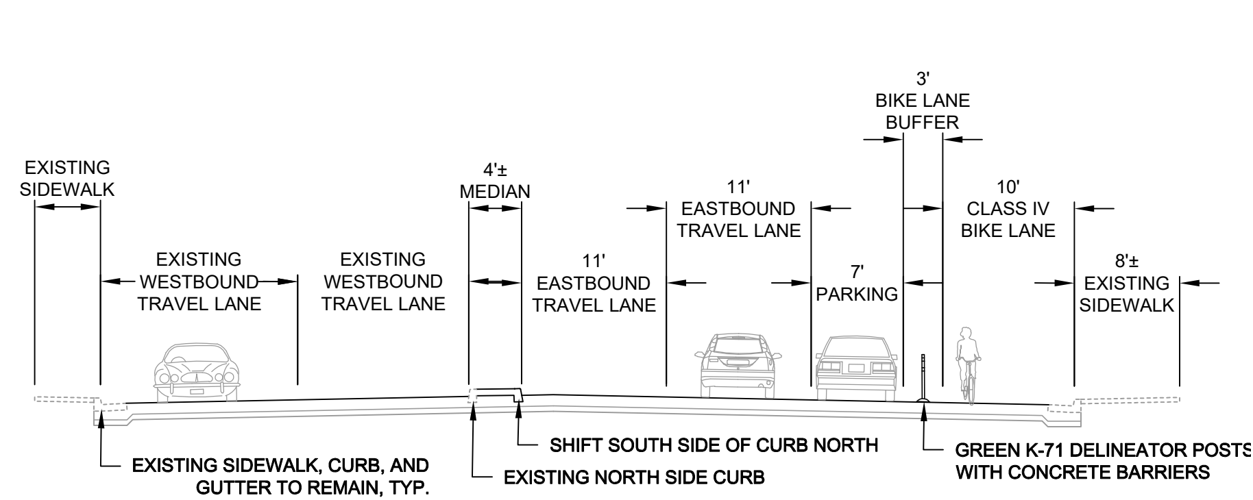
TYPICAL SECTION BETWEEN WEST AND EAST STREET
