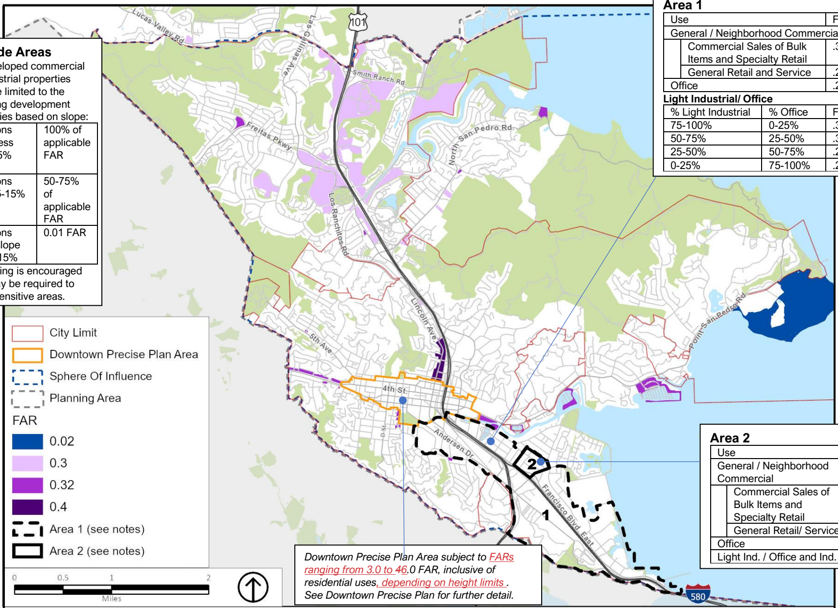
Figure 3-2: Floor Area Ratio (FAR) Limits
