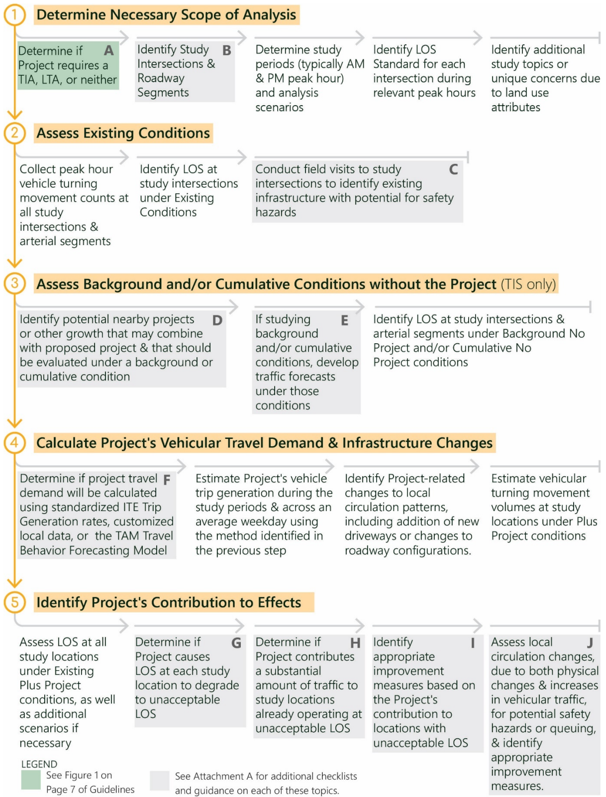
Figure 2: Flow Chart for Transportation Analysis and Documentation
