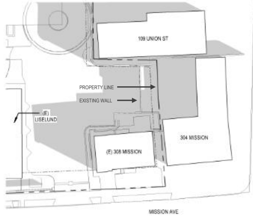
7 EXISTING - DECEMBER 21 @ 9:00 am 1" = 30'-0"
