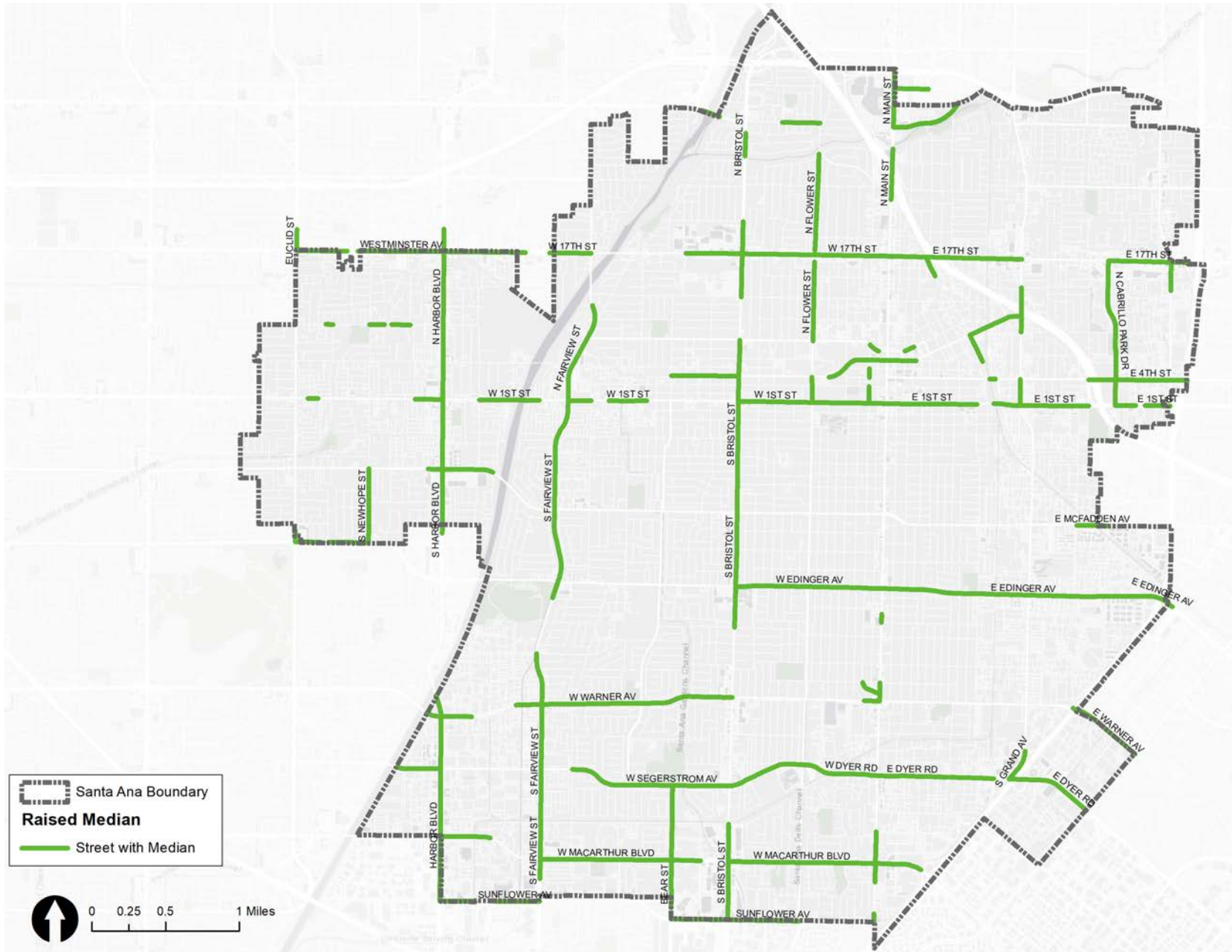
Figure 2-5: Raised Medians
