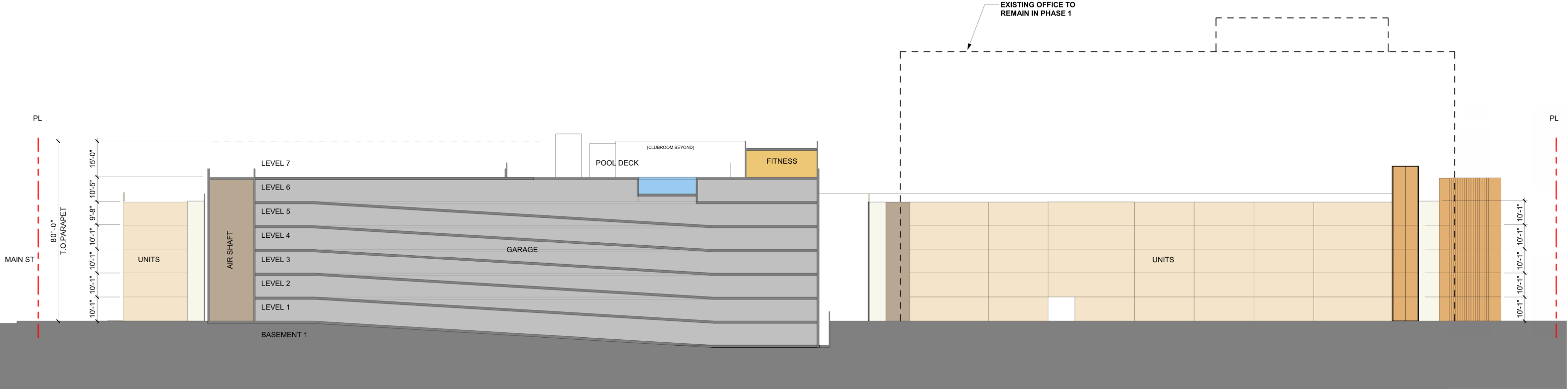
1) BUILDING SECTION - PHASE I & II
