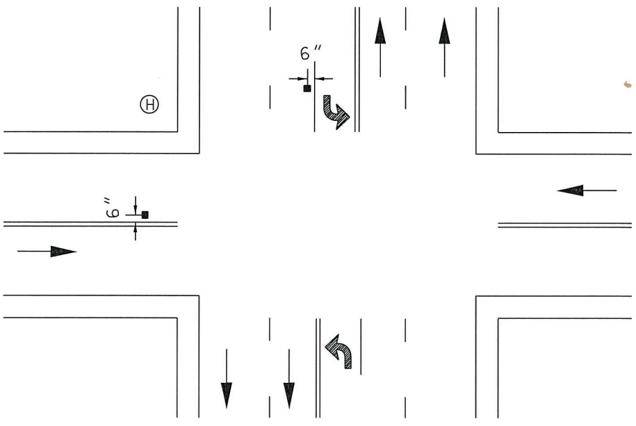
INTERSECTION WITH TURN LANES
