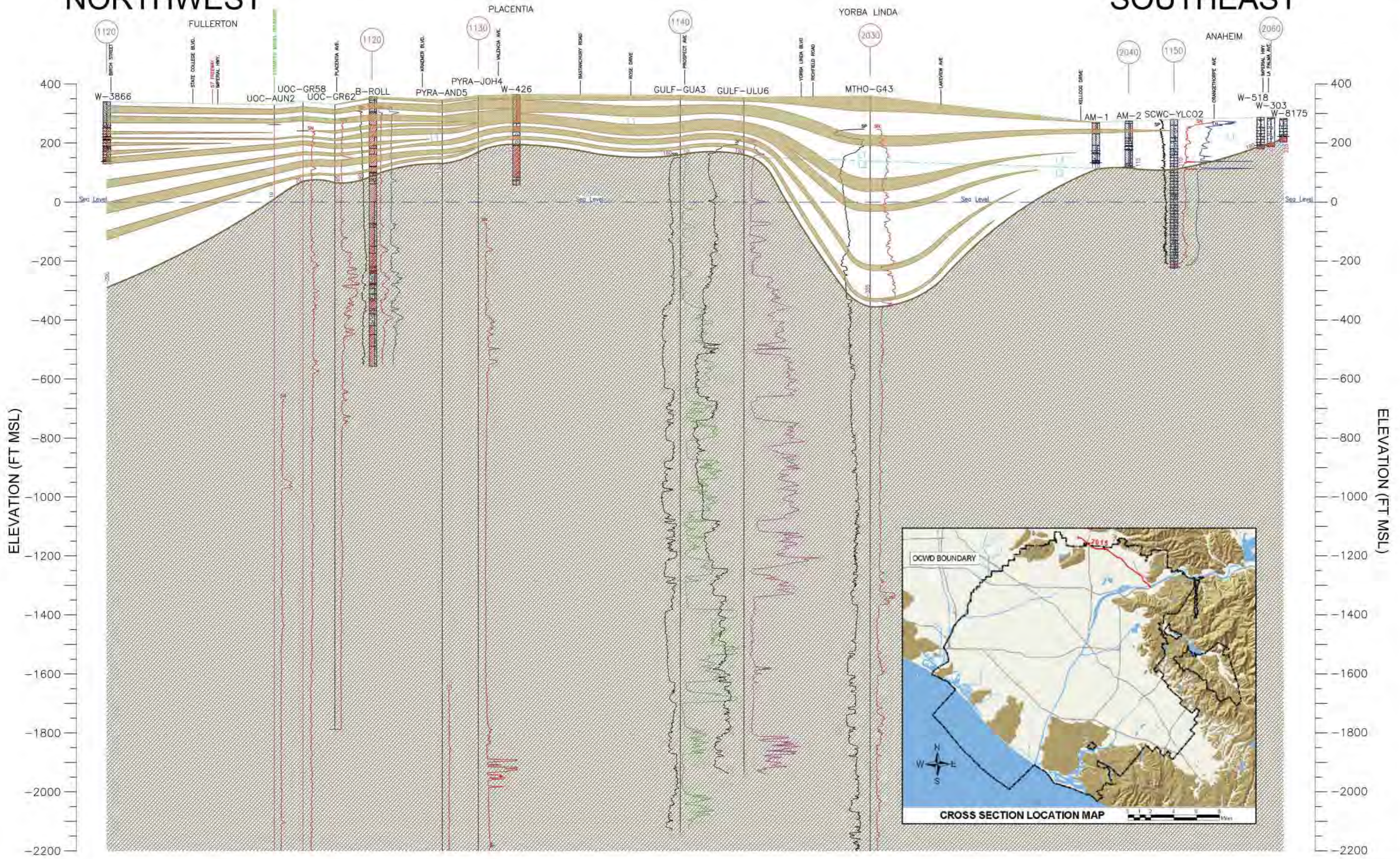
Figure 2-7: Cross Section 2015
