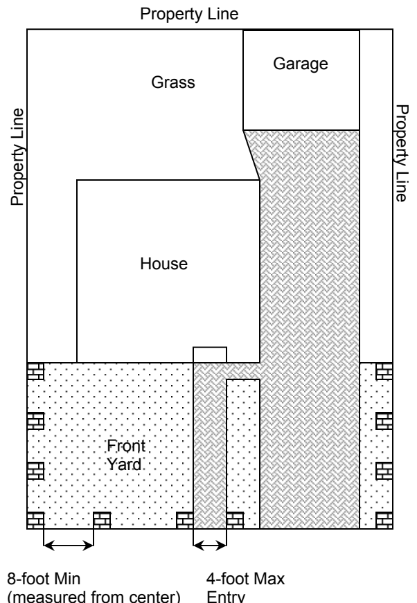
Example of Residential Site Plan-Non Corner Lot
