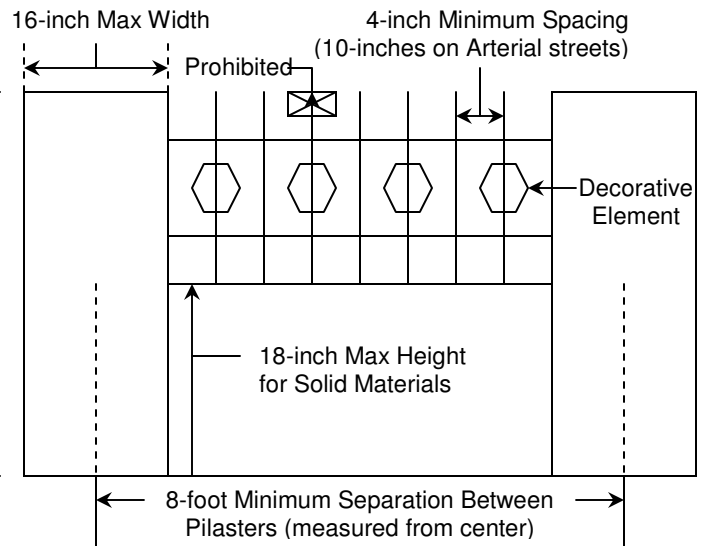
Example of Masonry Fence Design with Pilasters
