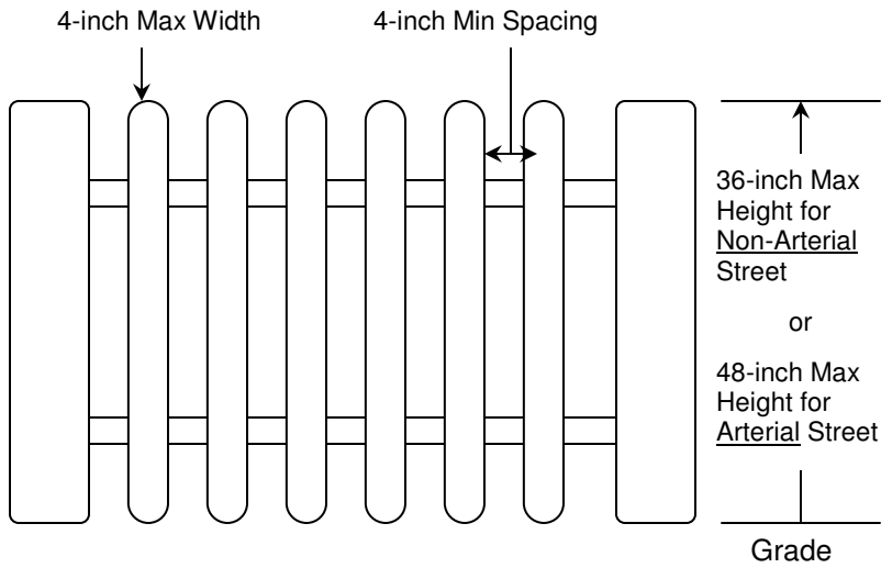
Example of Wood Picket/Wrought Iron Fence Design
