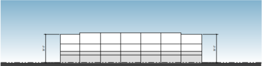
EAST ELEVATION
