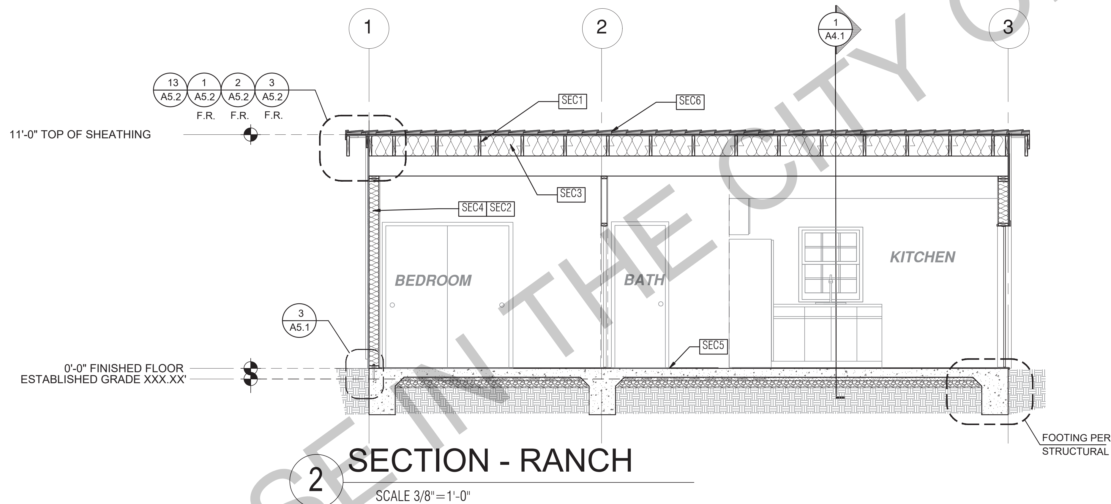
1 SECTION - RANCH SCALE 3/8" = 1'-0"
