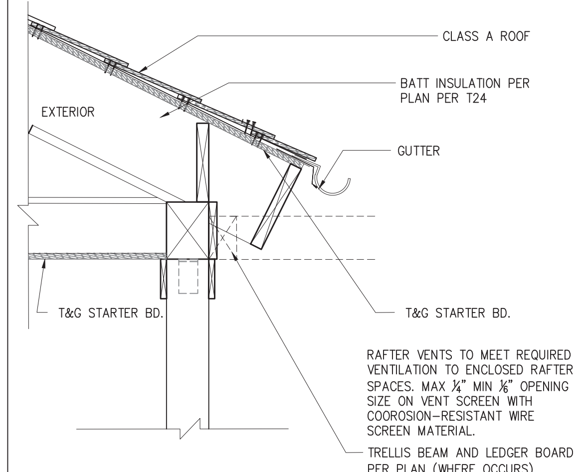
18 EAVE AT TRADITIONAL PORCH SCALE: 1"=1'-0"
