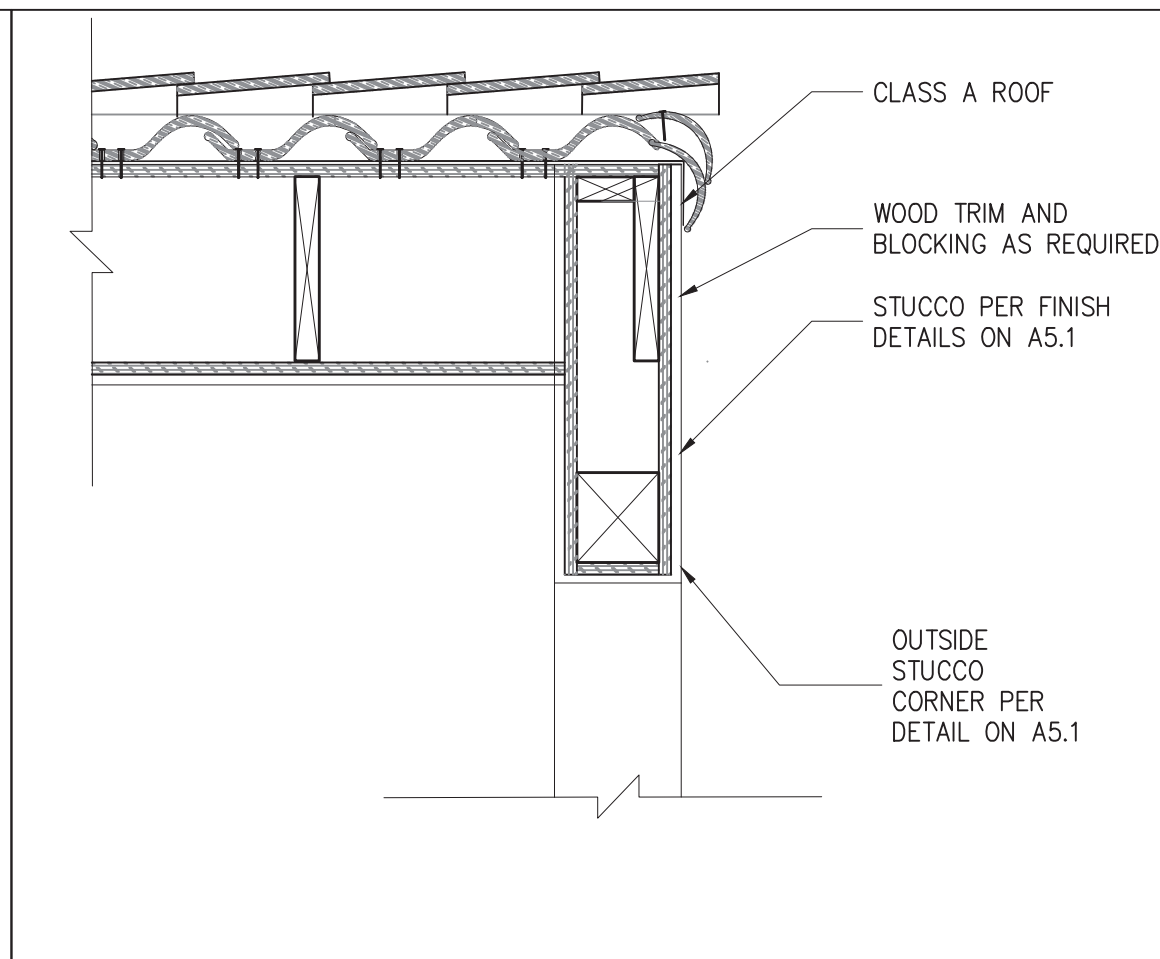
9 GABLE AT SPANISH PORCH SCALE: 1"=1'-0"
