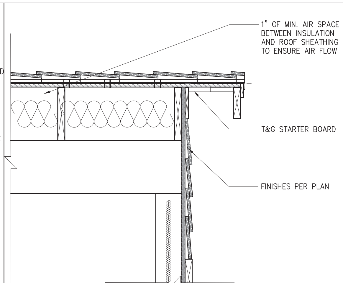
13 GABLE END AT RANCH & TRADITIONAL SCALE: 1"=1'-0"
