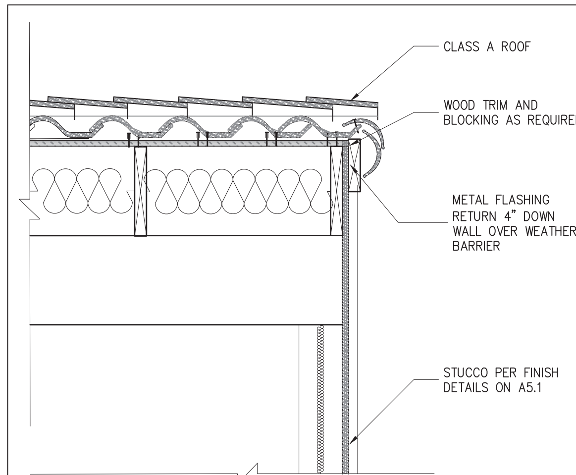
17 GABLE END AT SPANISH SCALE: 1"=1'-0"
