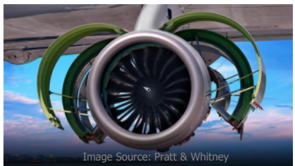
Ultra-high bypass geared turbofan engine
