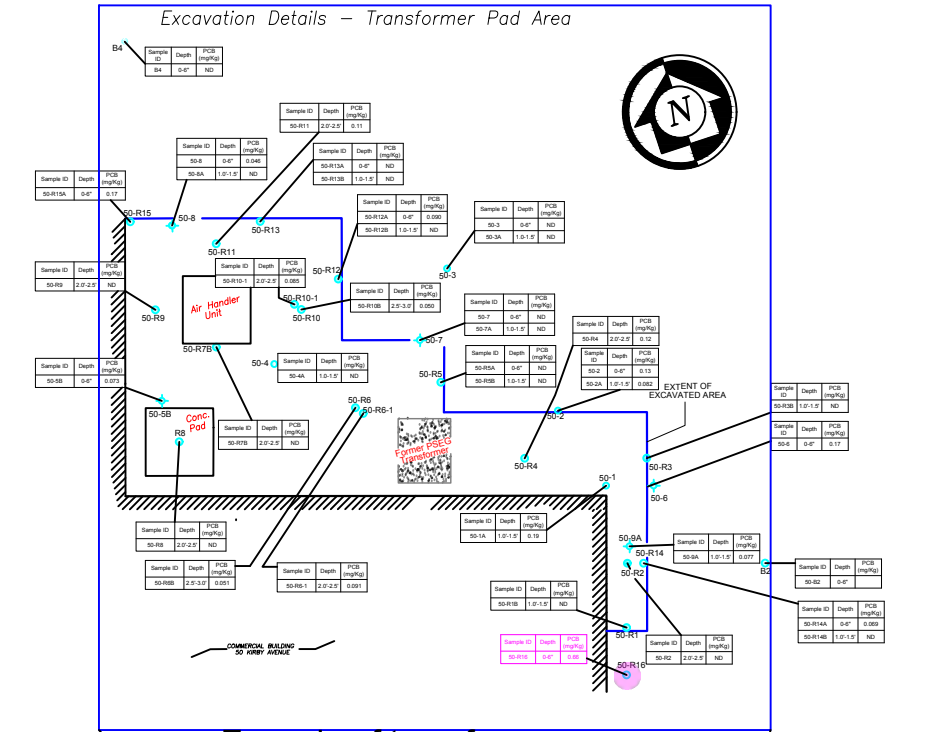
Zoom in of transformer area
