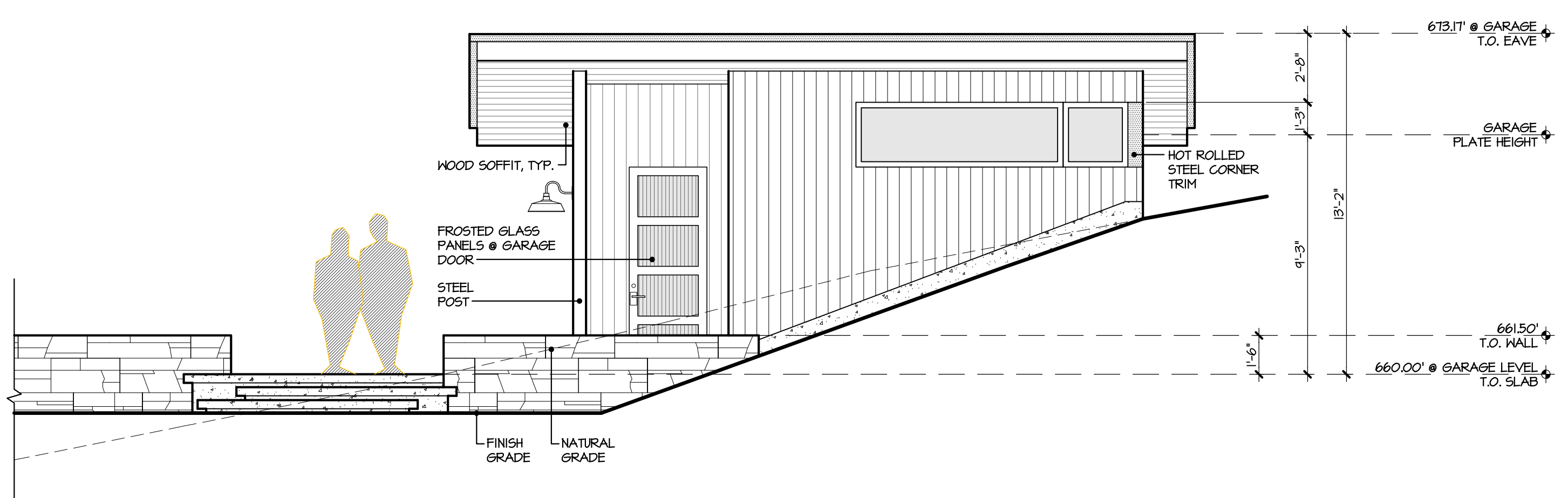
2 EAST ELEVATION GARAGE VIEW
