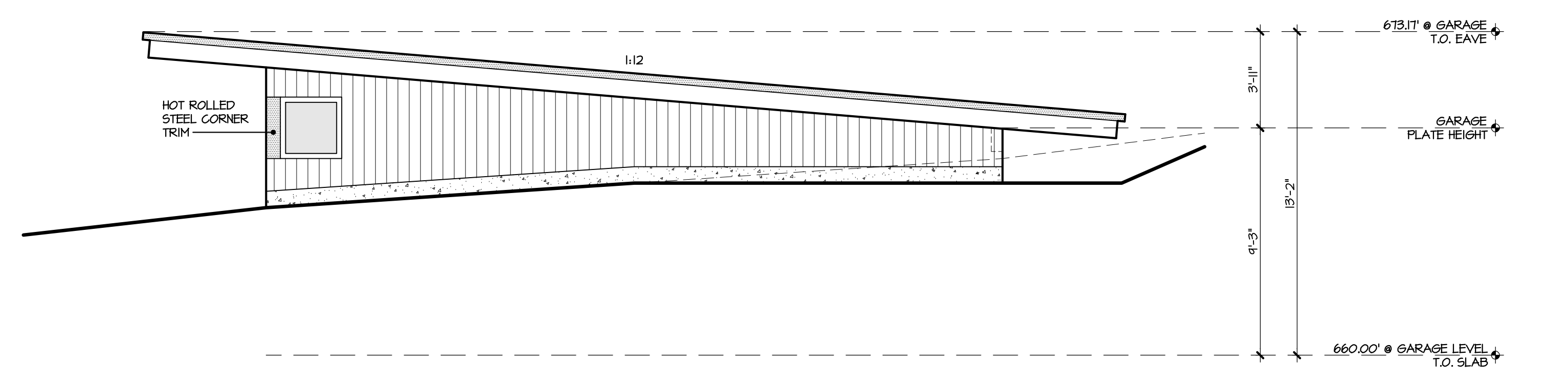
4 NORTH ELEVATION GARAGE VIEW
