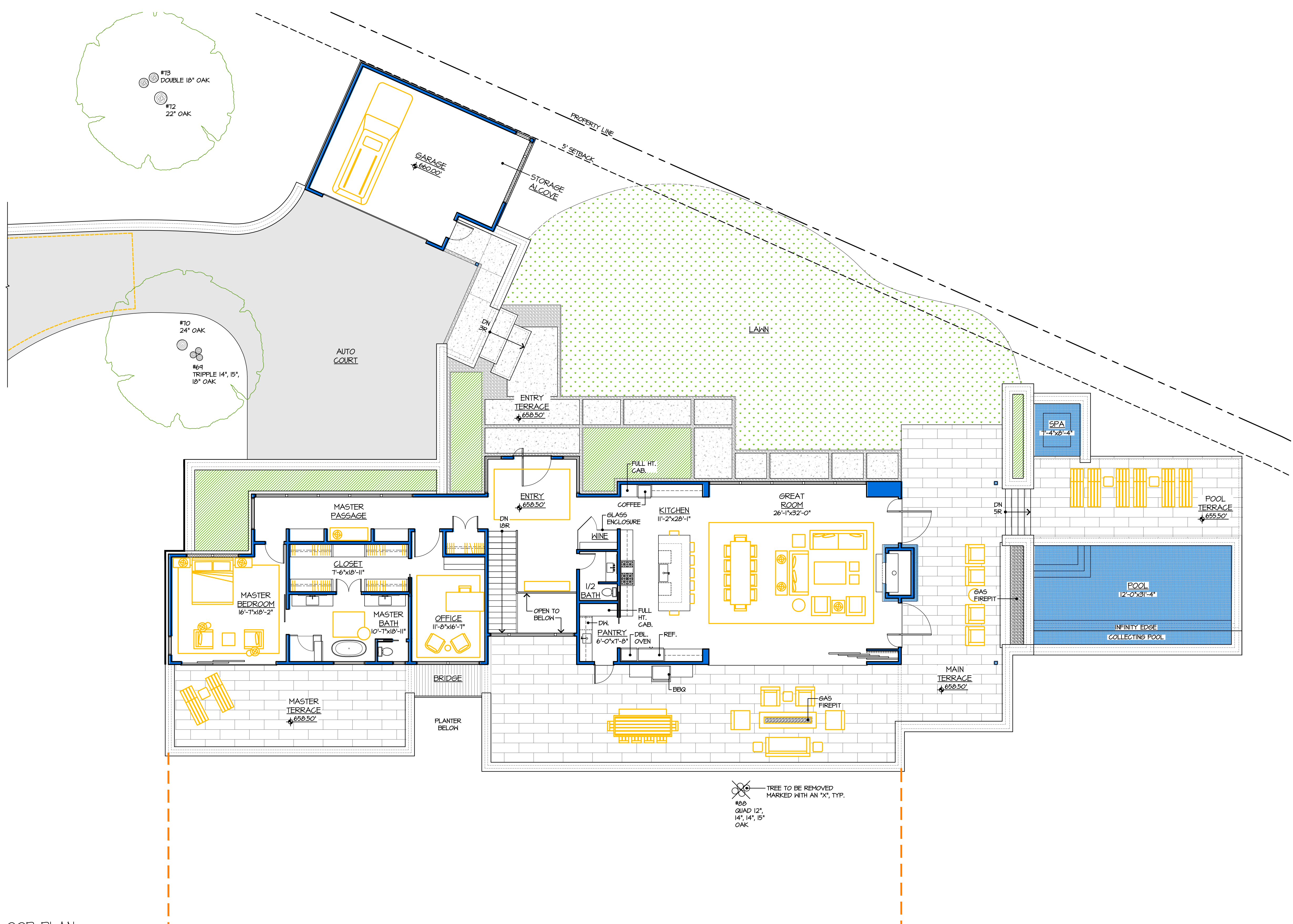
1 MAIN LEVEL FLOOR PLAN
