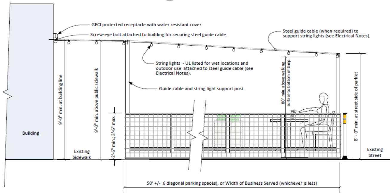
2 Street Elevation – Raised Parklet with String Lights SP-06
